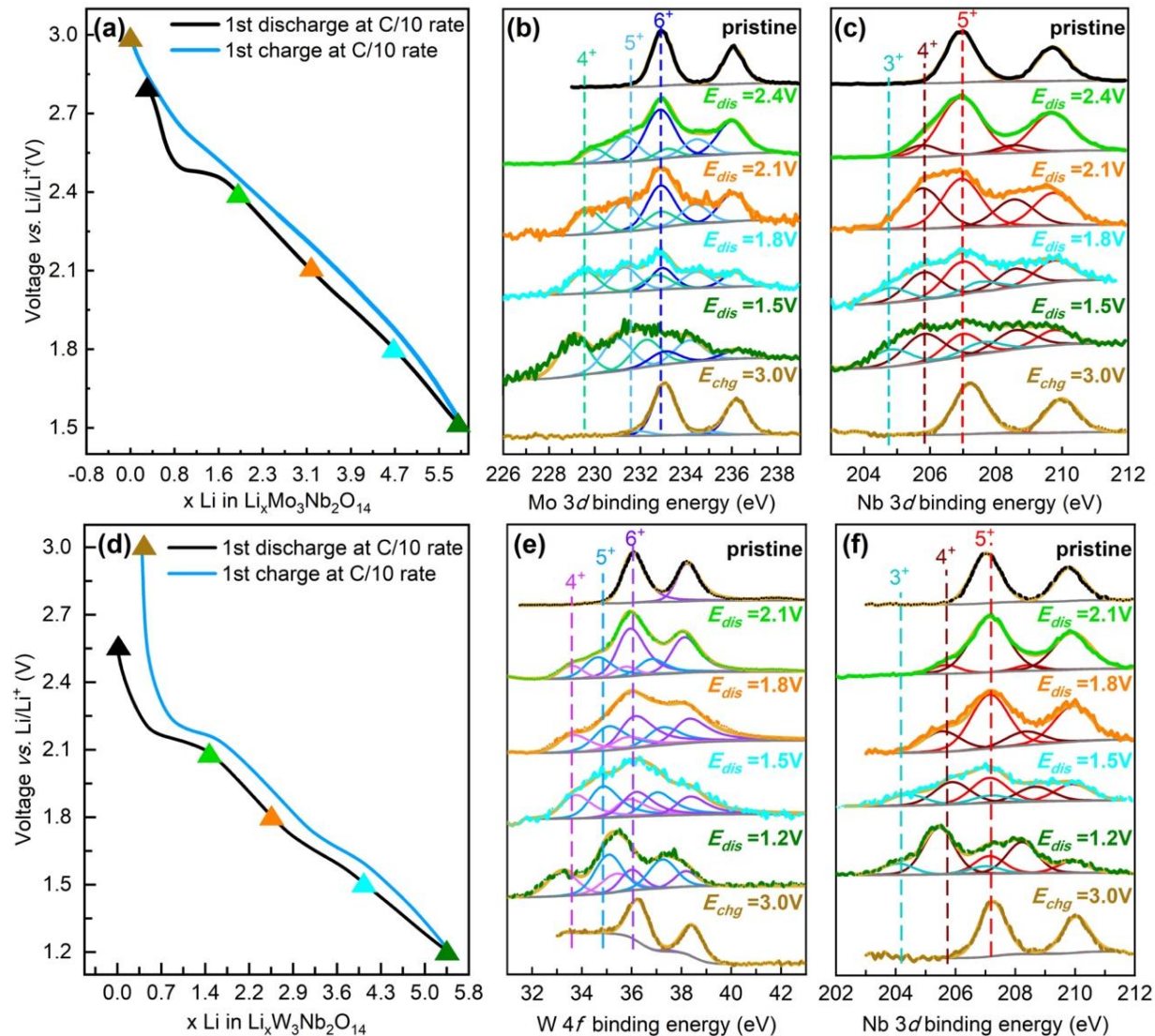
Figure 5. (a) The first galvanostatic discharge and charge for Li insertion in Mo 3 Nb 2 O 14 and the potentials corresponding to the XPS spectra in the Mo 3d binding energy region (b) and Nb 3d binding energy region (c). Similarly, (d) is the first galvanostatic discharge and charge for Li insertion in W 3 Nb 2 O 14 and the potentials corresponding to XPS spectra in the W 4f binding energy region (e) and Nb 3d binding energy region. The spin-orbit splitting contributes to the duplicate peaks shown in Nb 3d, Mo 3d, and W4f states. For simplification, the lower binding energy peaks are marked for indicating the oxidation states of transition metals. All grey lines correspond to the Shirley-type fitting background.
