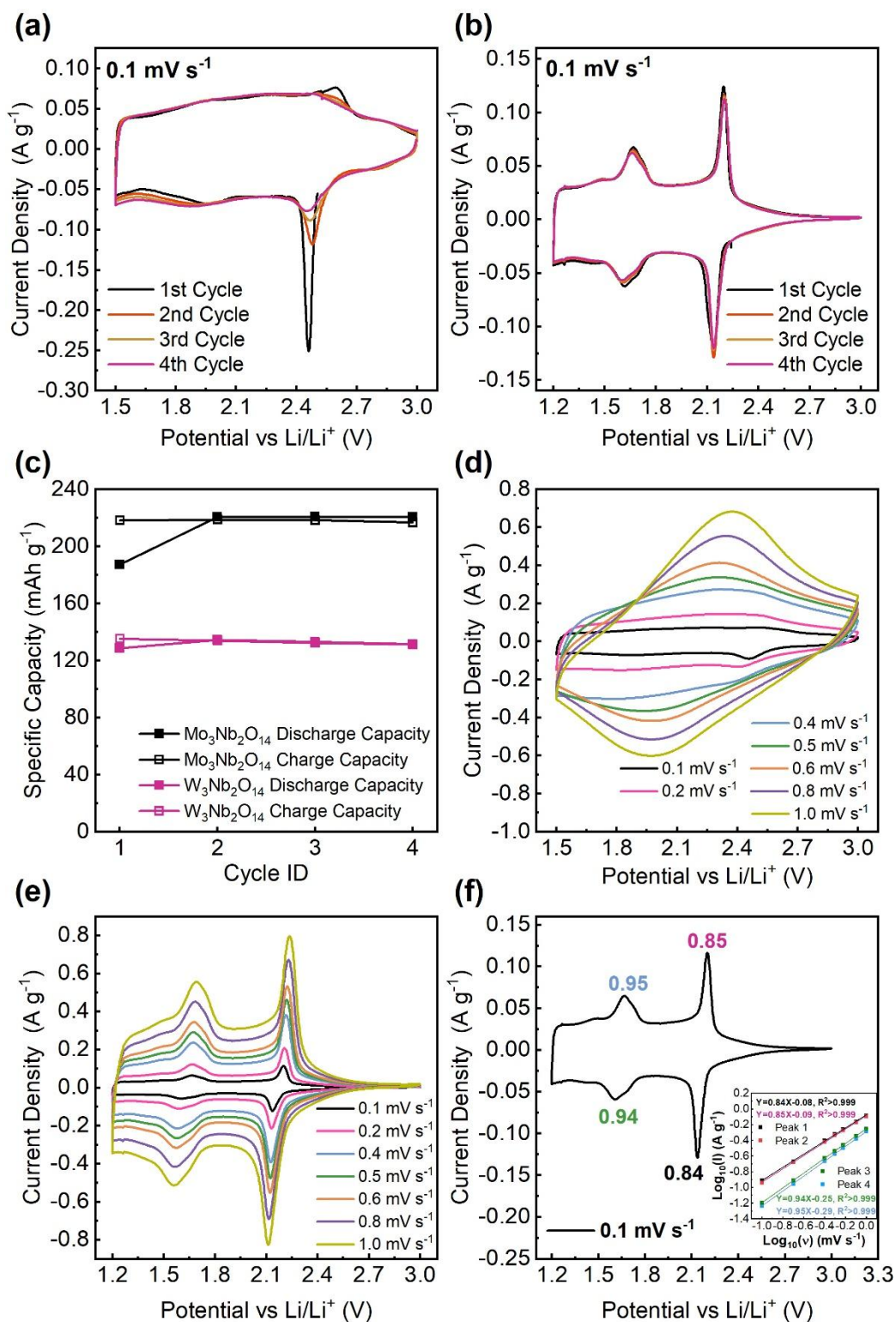
Figure 4. Cyclic voltammetry (CV) of (a) \text{Mo}_3\text{Nb}_2\text{O}_{14} and (b) \text{W}_3\text{Nb}_2\text{O}_{14} at a scan rate of 0.1 \text{ mV s}^{-1} for the first 4 cycles. (c) The comparison of calculated discharged and charged specific capacity from CV at a scan rate of 0.1 \text{ mV s}^{-1} for the first 4 cycles between \text{Mo}_3\text{Nb}_2\text{O}_{14} and \text{W}_3\text{Nb}_2\text{O}_{14} ; the CV curves of (d) \text{Mo}_3\text{Nb}_2\text{O}_{14} and (e) \text{W}_3\text{Nb}_2\text{O}_{14} at
