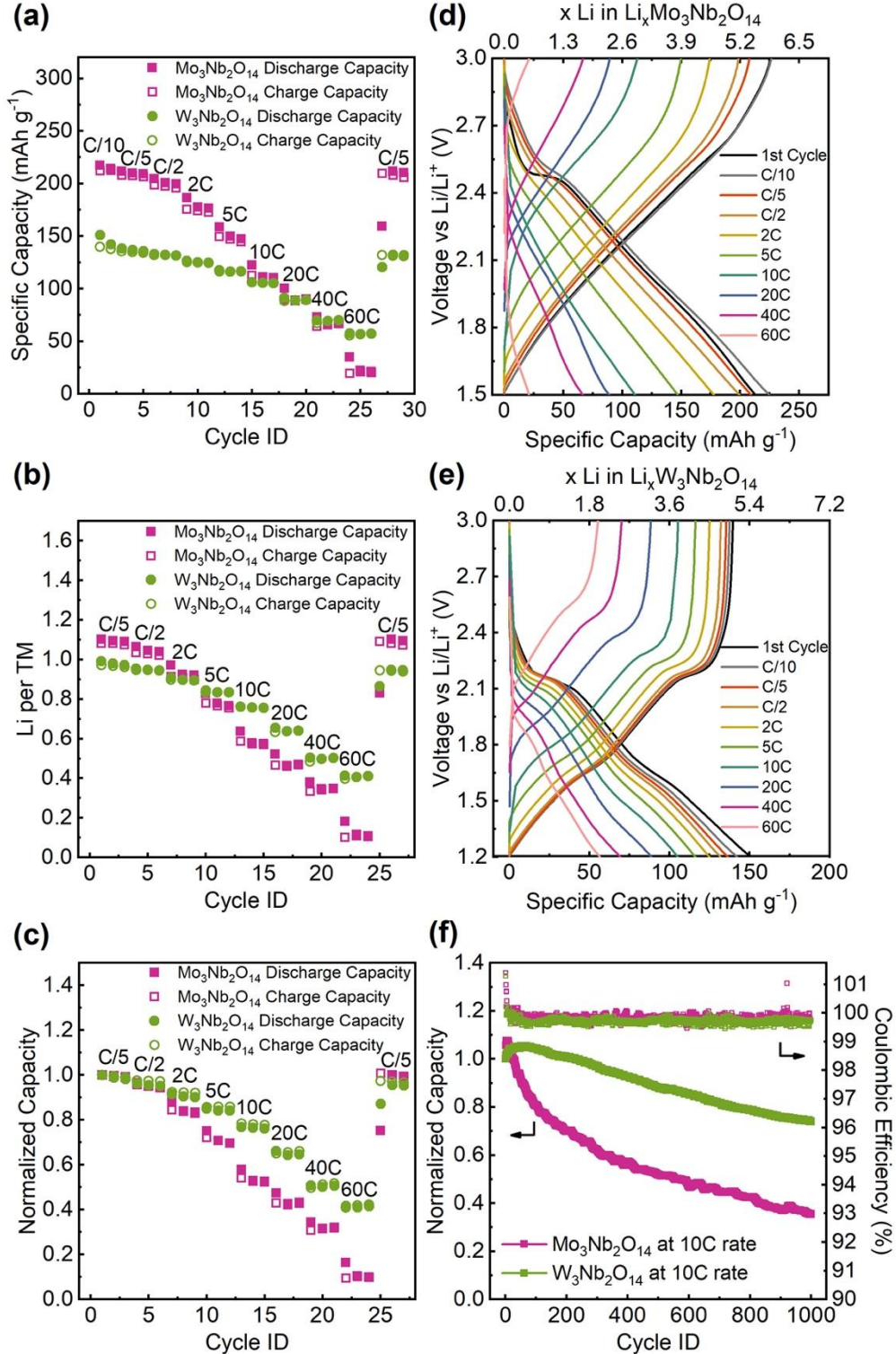
Figure 3. (a-c) Comparison of variable rate galvanostatic cycling in terms of specific capacity, lithium per transition metal and normalized capacity at C/5 between \text{Mo}_3\text{Nb}_2\text{O}_{14} and \text{W}_3\text{Nb}_2\text{O}_{14} ; the galvanostatic curve of voltage as a function of specific capacity for (d) \text{Mo}_3\text{Nb}_2\text{O}_{14} and (e) \text{W}_3\text{Nb}_2\text{O}_{14} ; (f) Comparison of long-term galvanostatic cycling at 10C for 1000 cycles for \text{Mo}_3\text{Nb}_2\text{O}_{14} and \text{W}_3\text{Nb}_2\text{O}_{14} . The specific capacity values for the first cycle at 10C for each material represent the reference values for the normalized capacity.
