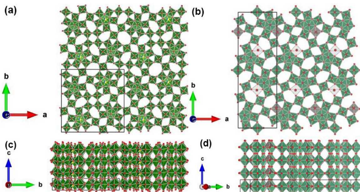
Figure 1. The unit cell of (a) \text{Mo}_3\text{Nb}_2\text{O}_{14} or (b) \text{W}_3\text{Nb}_2\text{O}_{14} projected down the c axis; the \text{W}_3\text{Nb}_2\text{O}_{14} structure is depicted based on CIF file of \text{W}_{10.7}\text{Nb}_{6.3}\text{O}_{47} . The unit cell of (c) \text{Mo}_3\text{Nb}_2\text{O}_{14} or (d) \text{W}_3\text{Nb}_2\text{O}_{14} projected down the a direction. The bipyramid pentagonal sites and octahedral sites in \text{Mo}_3\text{Nb}_2\text{O}_{14} are randomly occupied by Mo and Nb. The \text{W}_3\text{Nb}_2\text{O}_{14} possesses the same tunnel structure as \text{W}_{10.7}\text{Nb}_{6.3}\text{O}_{47} but with a different occupancy of transition metal, which is described in Figure S4. The crystal structures were depicted using VESTA.
