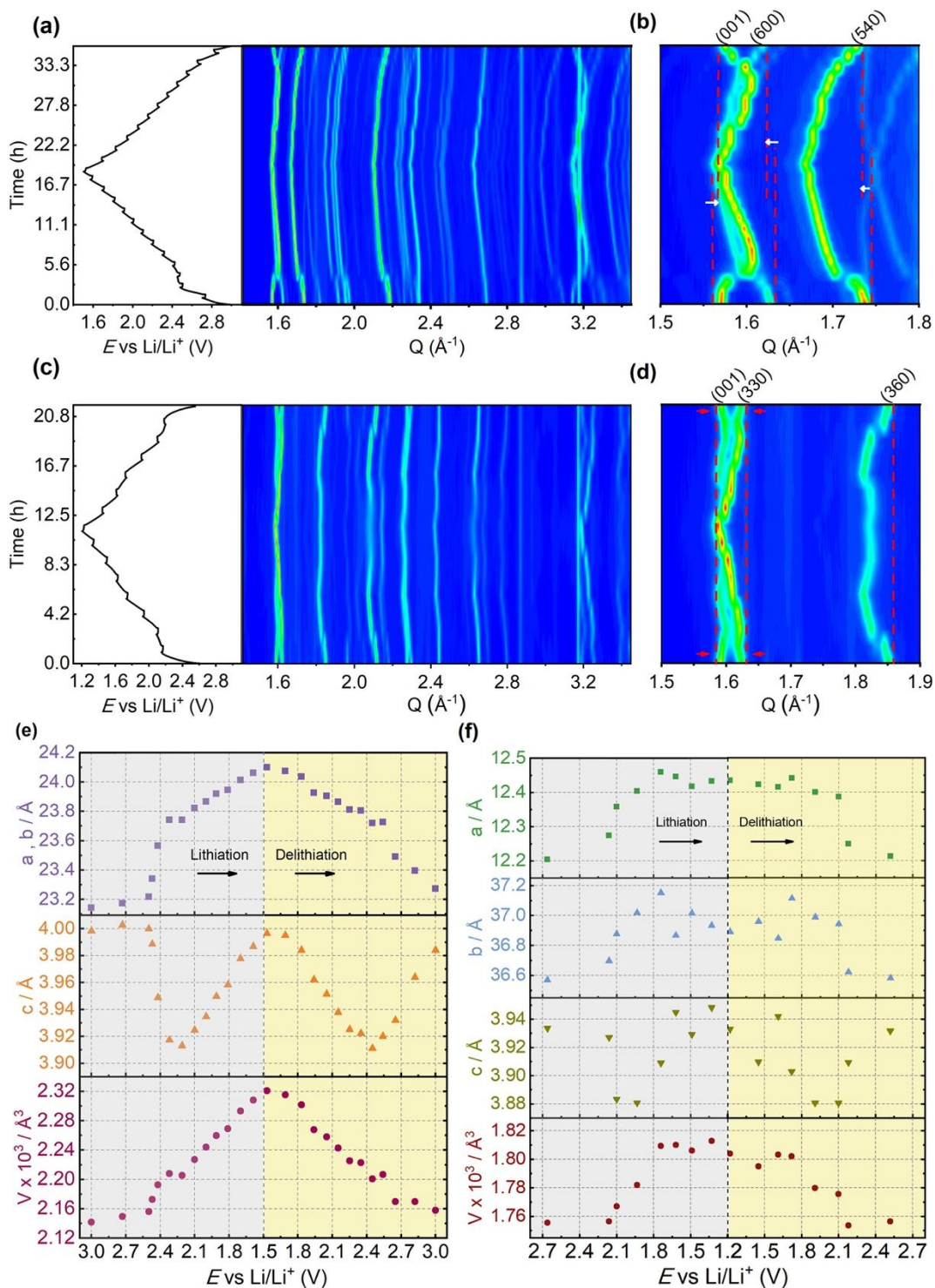
Figure 6. In-situ XRD patterns of (a) \text{Mo}_3\text{Nb}_2\text{O}_{14} discharged to 1.5 V and charged to 3.0 V at a C/10 rate and (c) \text{W}_3\text{Nb}_2\text{O}_{14} discharged to 1.2 V and charged to 3.0V at a C/10 rate; Selected Q range in In-situ XRD pattern of (b) (001), (600) and (540) plane of \text{Mo}_3\text{Nb}_2\text{O}_{14} or (d) (001), (330) and (360) plane of \text{W}_3\text{Nb}_2\text{O}_{14} ; Resolved lattice parameters and unit cell volume variations during discharging and charging at C/10 rate from Le Bail refinement of (e) \text{Mo}_3\text{Nb}_2\text{O}_{14} or (f) \text{W}_3\text{Nb}_2\text{O}_{14} .
