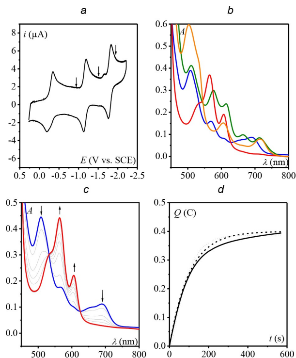
Figure 5. (a) FeTPPCl 0.4 mM in DMF + 0.1 M NBu 4 PF 6 under argon: CV at 0.1 V/s on a 3 mm diameter glassy carbon electrode. (b) UV-vis spectra (Q-bands, l = 1 mm) initial (blue) and after application of constant potential -0.92 (red), -1.42 (green) and -1.87 (orange) V vs. SCE. (c) Time evolution of UV-vis spectra during application of a constant potential -0.92 V vs. SCE; the initial spectrum is in blue and the final spectrum is in red. (d) Time evolution of the charge passed during application of a constant potential -0.92 V vs. SCE. Dashed line: fitting with Q = Q_{\max}[1 - \exp(-t/t_{\text{eff}})] . Dotted line: time evolution of the normalized absorbance at 690 nm according to: Q_{\max}[1 - (A_{690} - A_{690,t=0})/(A_{690,t=0} - A_{690,t=\infty})] .
