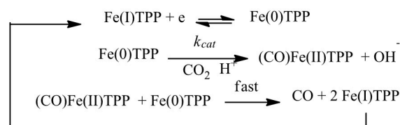
Scheme 2. Reaction scheme for CO 2 electroreduction catalyzed by FeTPP.
