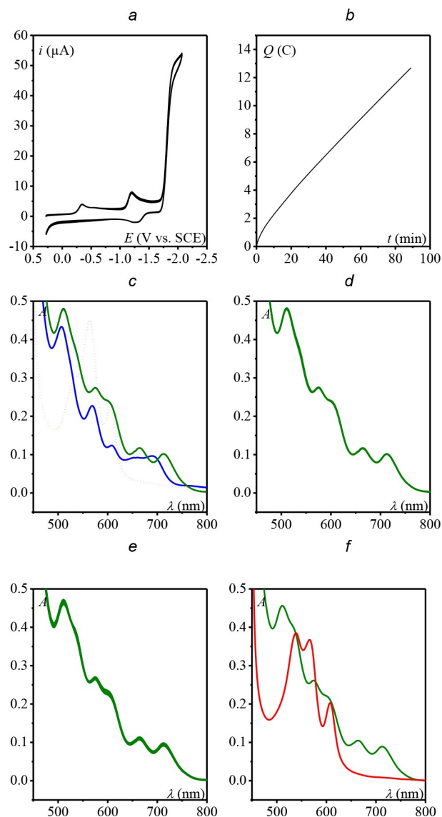
Figure 6. FeTPPCl 0.4 mM in DMF + 0.1 M NBu 4 PF 6 at 0.1 V/s on a 3 mm diameter glassy carbon electrode under CO 2 and with 6.7 mM of PhOH: (a) CV; (b) Time evolution of the charge passed during application of a constant potential -1.82 V vs. SCE (18 mL solution); (c) UV-vis spectra (Q-bands, l = 1 mm) during application of a constant potential -1.82 V vs. SCE. Blue: initial spectrum, dotted red: spectrum after 3 min, green: spectrum after 30 min. (d) Overlay of UV-vis spectra during application of a constant potential -1.82 V vs. SCE between t = 20 min to t = 90 min (one spectrum / 10 s). (e) Overlay of UV-vis spectra during application of a constant potential -1.52 V vs. SCE (one spectrum / 10 s) after 90 min electrolysis at -1.82 V vs. SCE. (f) UV-vis spectra before (green) and after (red) application of a constant potential at -0.72 V to the solution obtained after (e).
