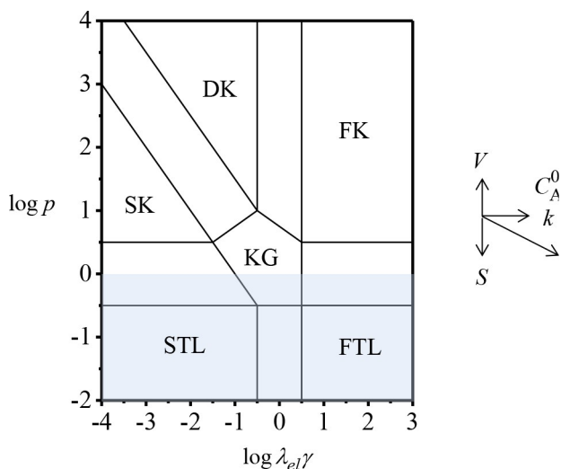
Figure 2. Schematic zone diagram for CPE as a function of the two dimensionless parameters p = \frac{V/S}{\delta} and \lambda_{el}\gamma = \frac{kC_A^0}{D/\delta^2} . KG: general case (equations (5) and (6)). SK: slow catalysis. FK: fast catalysis. DK: diffusion case. The light blue region corresponds to thin layer. STL: thin layer slow catalysis. FTL: thin layer fast catalysis. The arrows summarize how the variations of the parameters move the system from one zone to the other. Zones without names are transition zones.
