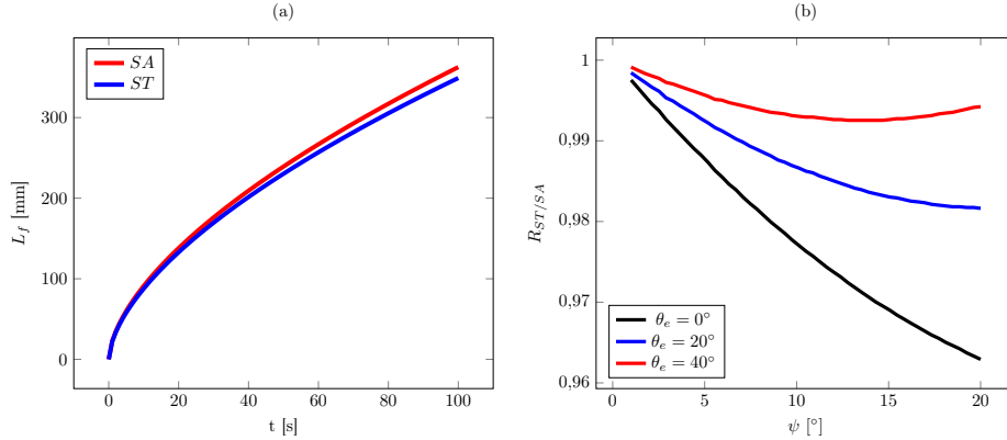
FIGURE 2: (a) Evolution of the film extension for an imposed volume flow rate; (b) Ratio of liquid film extensions as a function of \psi .
