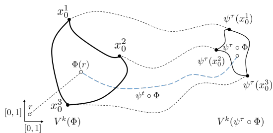
Fig. 1. Flow of a 2-contractive system. The initial submanifold of initial conditions, described by \Phi , is some surface with points at x_0^1, x_0^2 and x_0^3 . The volume of this submanifold V^k(\cdot) decreases exponentially along the trajectories of the system.
