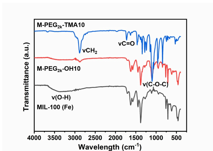
Figure S10. ATR-FTIR spectra of the MIL-100 (Fe) (bottom, black curve), M-PEG 2k -OH10 (middle, red curve), and M-PEG 2k -TMA10 (top, blue curve) solid samples obtained after the treatments summarized in the experimental section to obtain solid powders. The assignments of the main bands are indicated in the figure.
