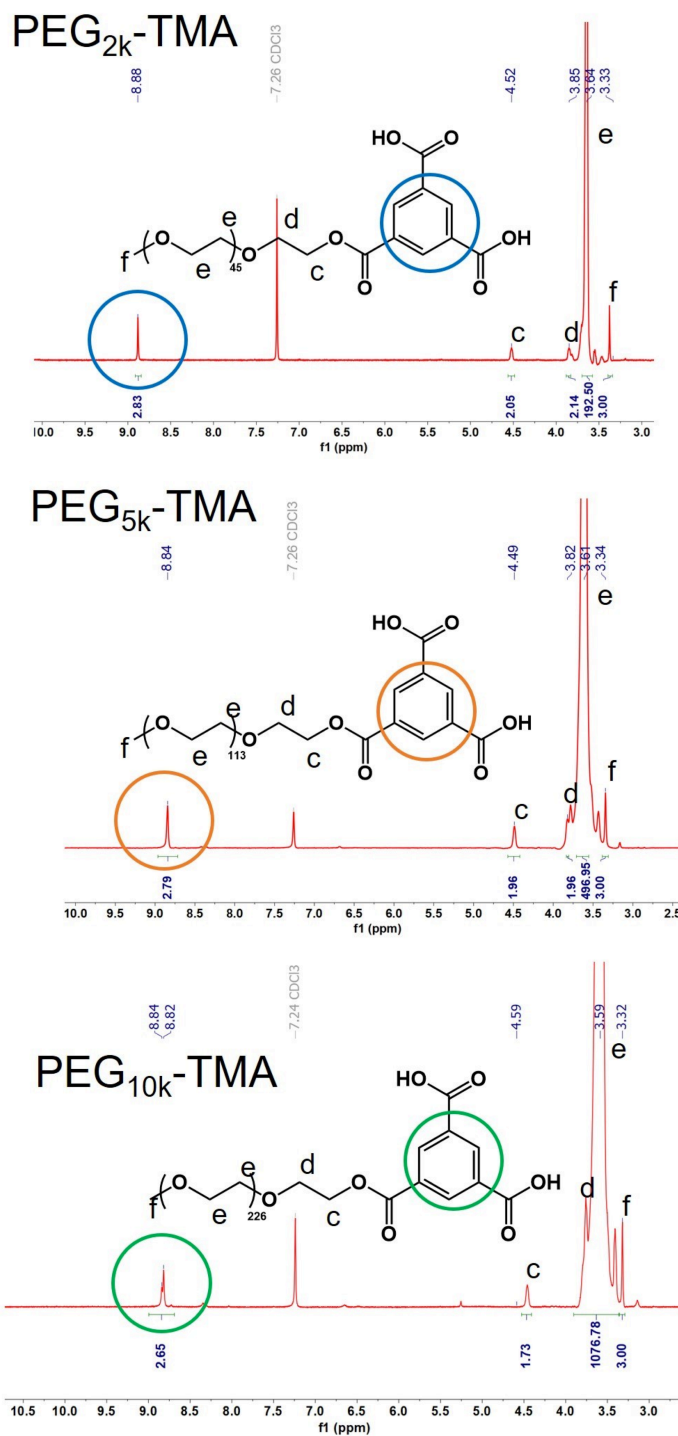
Figure S1. ^1\text{H} NMR spectra of PEG 2k -TMA, PEG 5k -TMA and PEG 10k -TMA in CDCl 3 .
