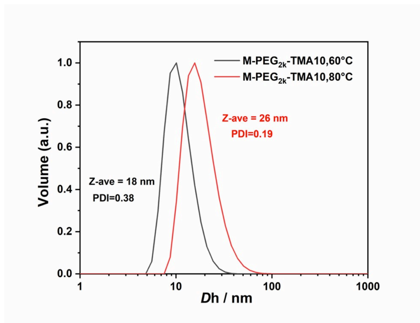
Figure S11. DLS volume-averaged distribution for M-PEG 2k -TMA10 particles synthesized at 60°C and 80°C, respectively (after a 1:4 dilution of the initial reaction mixture and filtration, see experimental section). Attempts at 20 and 40°C led to very large distributions whose parameters could not be reliably measured by our DLS equipment.
