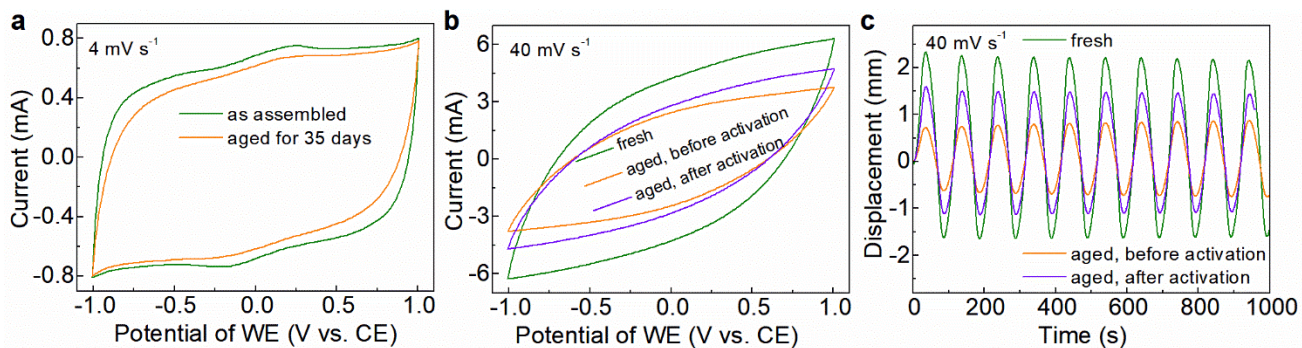
Figure S18. Effect of aging in ambient condition (21 °C, 65% relative humidity) on the performance of TBA-MXene based ECA: (a) CV curves at 4 \text{ mV s}^{-1} before and after 35-day aging; (b) CV curves at 40 \text{ mV s}^{-1} before and after 35-day aging. The activation was done by running a CV at 4 \text{ mV s}^{-1} for 10 cycles; (c) Actuation displacement of fresh and aged device at 40 \text{ mV s}^{-1} under a triangle wave of \pm 1 \text{ V} and 0.01 \text{ Hz} .
