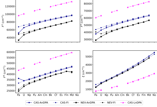
Figure 4: Slater-Condon parameters F^2 , F^4 and F^6 and the spin-orbit parameter \zeta for the An(III) free ions (dotted, from 13 ) and the [\text{An}^{\text{III}}(\text{DPA})_3]^{3-} (plain) series (CASSCF: blue, NEVPT2: black) and the [\text{Ln}^{\text{III}}(\text{DPA})_3]^{3-} (CASSCF, magenta, from 22 ) series.
