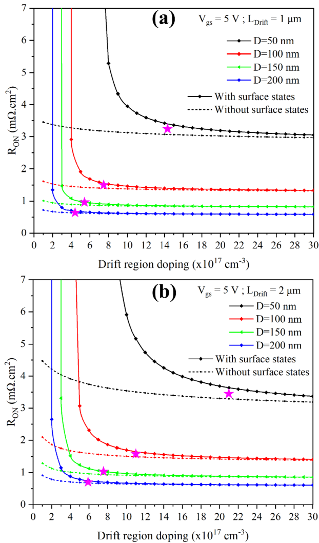
FIGURE 10. Evolution of the on-state resistance R_{ON} as a function of the doping level of the drift region, for a length L_{Drift} = 1 \mu\text{m} (a) and L_{Drift} = 2 \mu\text{m} (b).
