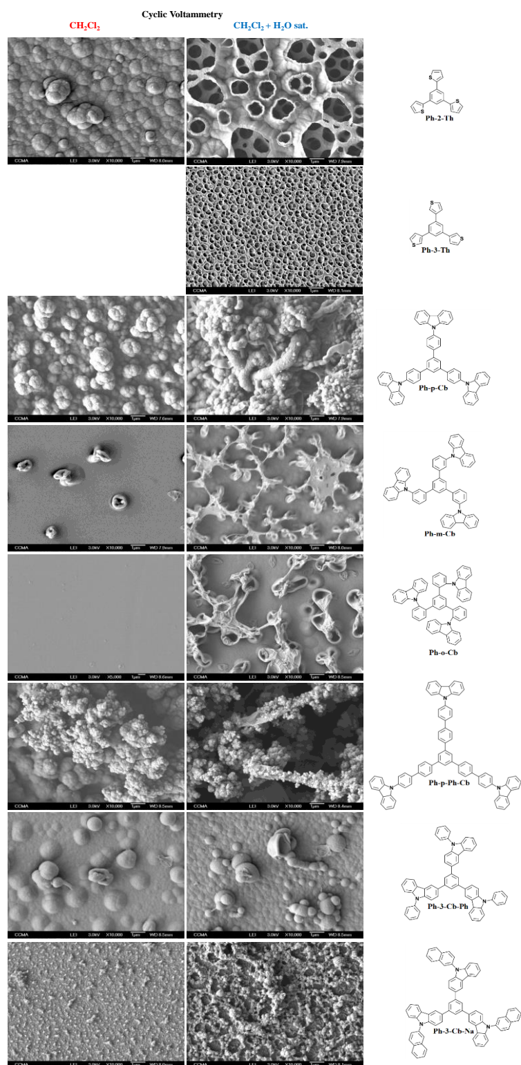
Figure 4. SEM images of electrodeposited surfaces from each monomer. 3 scans from -1 V to E^{ox} V with 0.1 M of Bu_4NClO_4 in CH_2Cl_2 or CH_2Cl_2 + H_2O sat. The scan rate was 20\text{ mV s}^{-1} .
