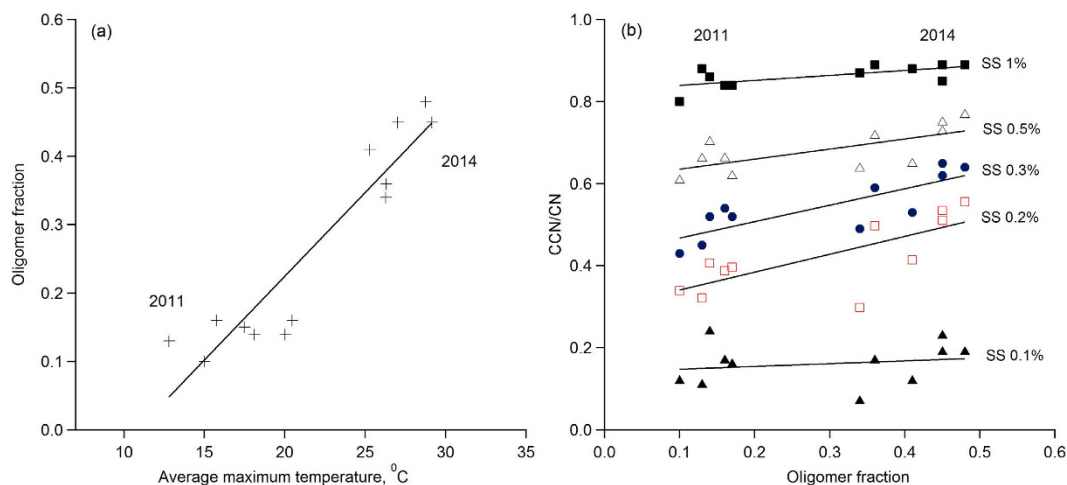
Figure 3. (a) Positive relationship between temperature and oligomer fraction in aerosol samples collected at Hyttiälä in summer 2011 and 2014. The oligomer fraction was determined as the average intensities of all oligomer peaks relative to the average intensity of all peaks in the mass spectrum of an individual sample. (b) Correlation of CCN/CN with oligomer fraction for all samples in 2011 and 2014 for supersaturations (SS) between 0.1% and 1%. For intermediate SS of 0.2 and 0.3% the CCN/CN ratio increases by up to 30–50%, i.e. from 0.34 to 0.49 for 0.2% SS and 0.47 to 0.61 for 0.3% SS.
