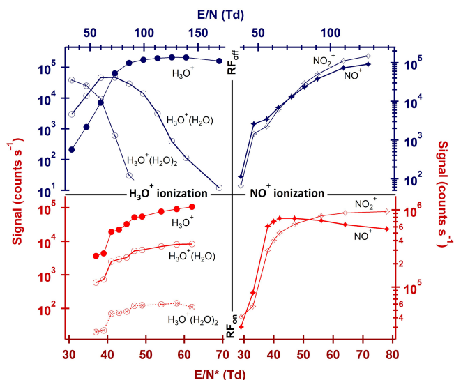
Figure 1. Typical ionizing species distribution as a function of the E/N ratio, in the two ionization modes with RF mode on and off. When the RF mode is on, E/N^* ratios were calculated taking into account only the contribution of the DC electric field while the additional input of the AC electric field remains difficult to estimate.
