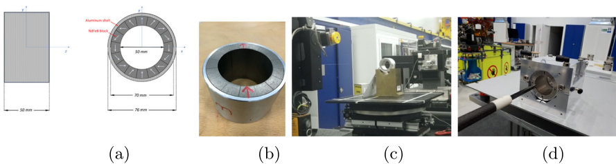
Fig. 4 The Mini.PAN magnets: a) Design sketch; b) Magnet prototype; c) Single magnet under integrated magnetic field measurement with stretched wire at CERN; d) 2-magnet assembly under 3D mapping of the magnetic field with Hall probe at CERN
