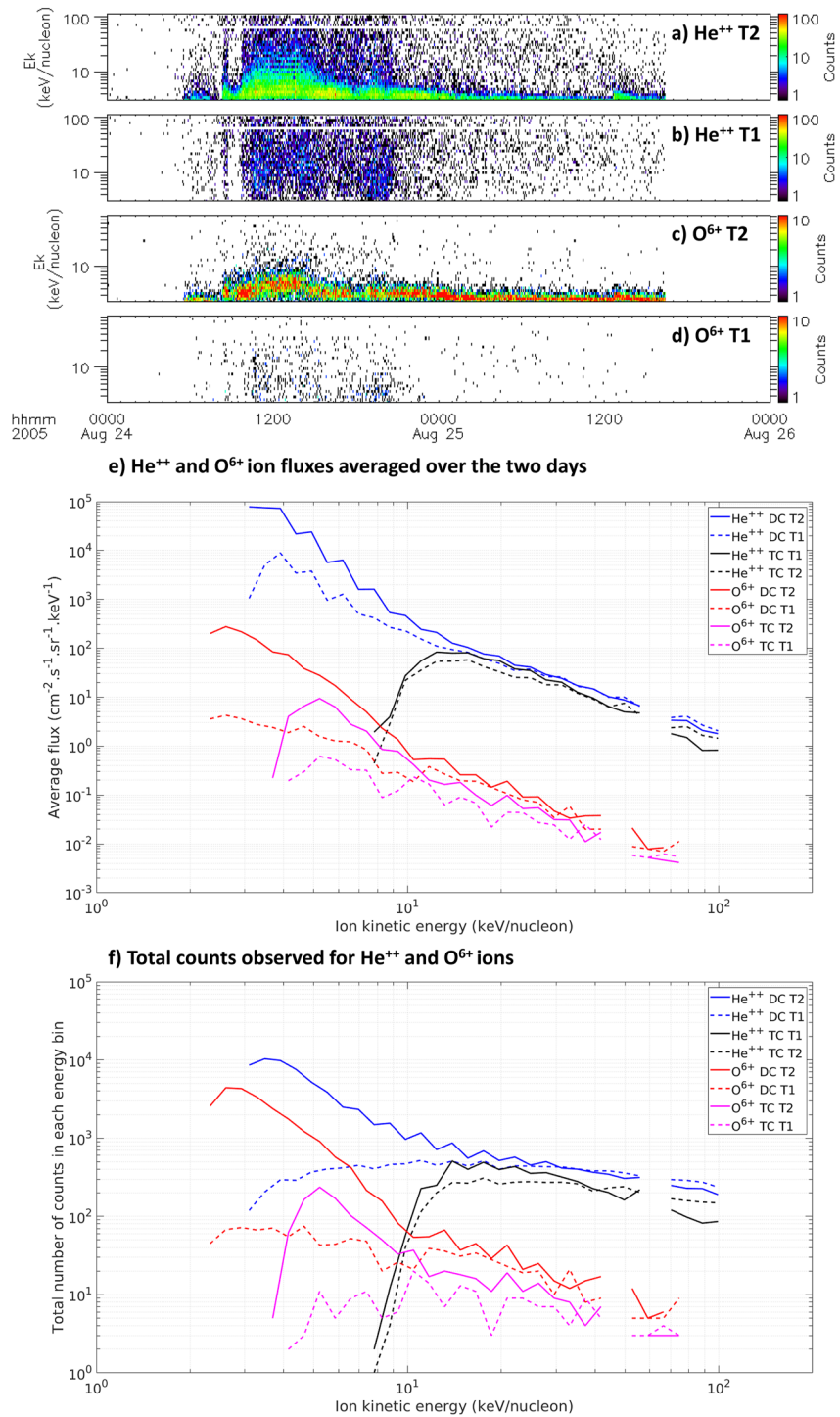
Figure 1. (a) Energy-time spectrogram of the He ++ ion counts observed by the in-ecliptic telescope 2 (labeled “T2”) of Wind-STICS in double coincidence with the native 3-min resolution. Ion counts are summed over all azimuthal sectors. (b) same as panel a but for the He ++ ion counts observed by the out-of-ecliptic telescope 1. (c) same as panel a but for O 6+ ions. (d) same as b but for O 6+ ions. (e) He ++ and O 6+ ion fluxes averaged over the 2-day period and observed in double and triple coincidence. (f) total number of counts corresponding to the fluxes of panel (e).
