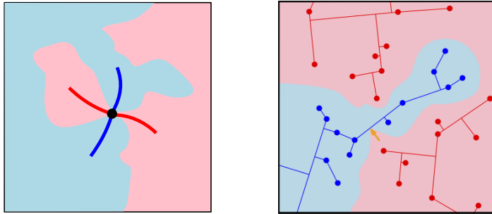
Figure 4: Left. Illustration of a double point in the frontier \mathcal{F}_\infty . Right. Can the frontier intersect the finite trees in the segment model (orange arrow)?
