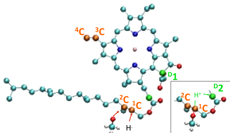
Figure 8 : Possible sites of methanol addition in orange, on a C=C double bond on the periphery of the chlorin ^3\text{C}-^4\text{C} or on the C=C the double bond of the phytol chain ^2\text{C}-^1\text{C} . In the insert, ^{\text{D}2} deuteration is followed by a proton transfer from ^1\text{C} localizing the negative charge on ^1\text{C} . The methanol addition in the combination ^{\text{D}1} - ^2\text{C} is shown below the chlorophyll molecule.
