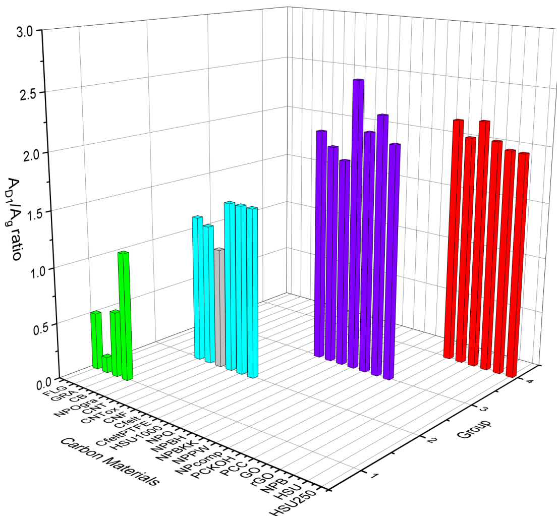
Figure S3. Comparison of the A_{D1}/A_G ratio obtained from the deconvolution of the Raman spectra of the studied carbon materials.
