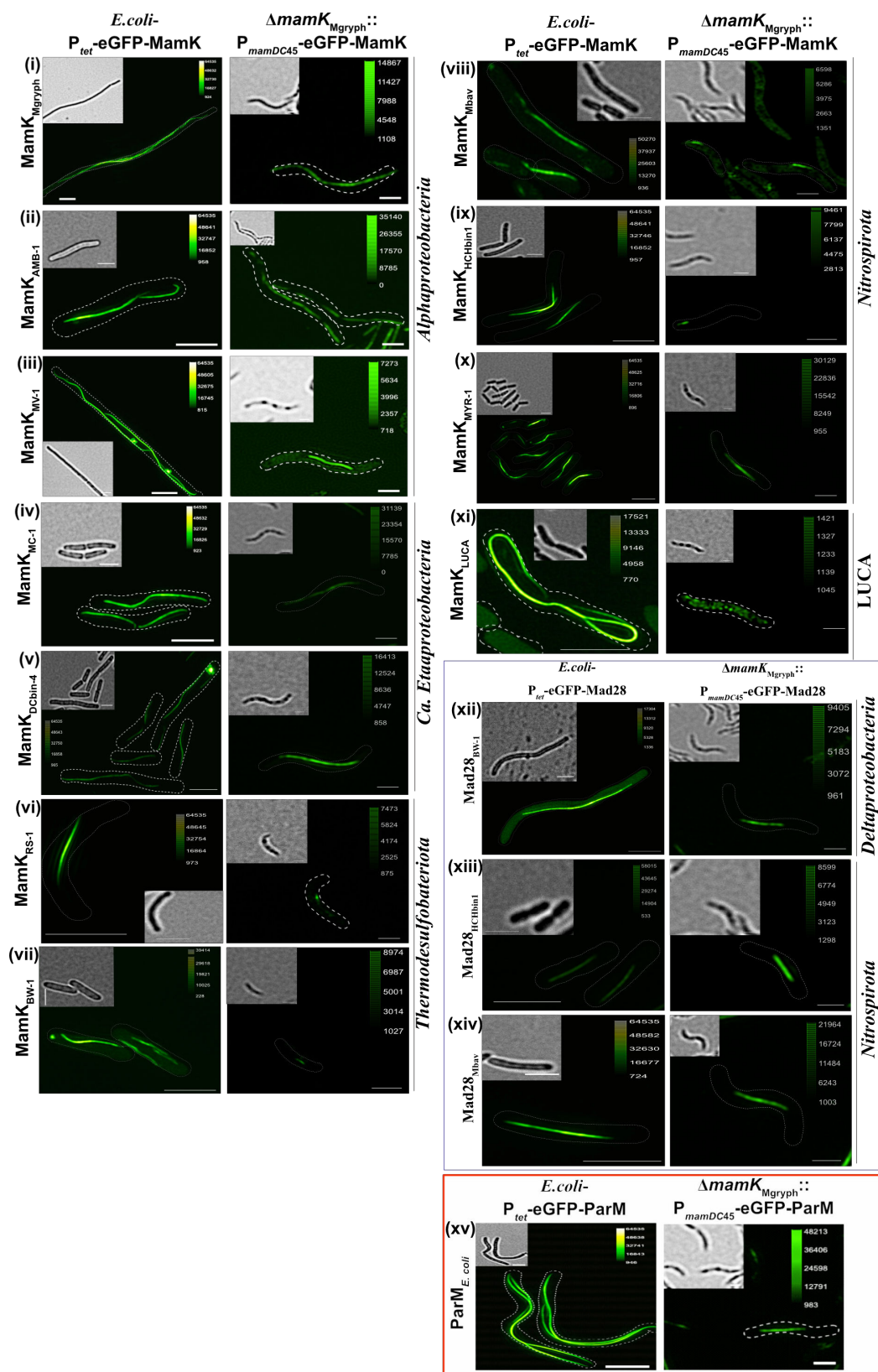
FIG 3 Three-dimensional structured illumination fluorescence microscopy micrographs (maximum intensity projection, brightfield as inset) of E. coli and Mgryp cells expressing EGFP-MamK/EGFP-Mad28 from diverse MTB and EGFP-ParM E.coli . Gene expression in E. coli was induced with anhydrotetracycline for 6 hours (50 ng/mL). In \Delta mamK Mgryp genes were constitutively expressed from P mamDC45 . Scale bars correspond to 1 \mu m.
