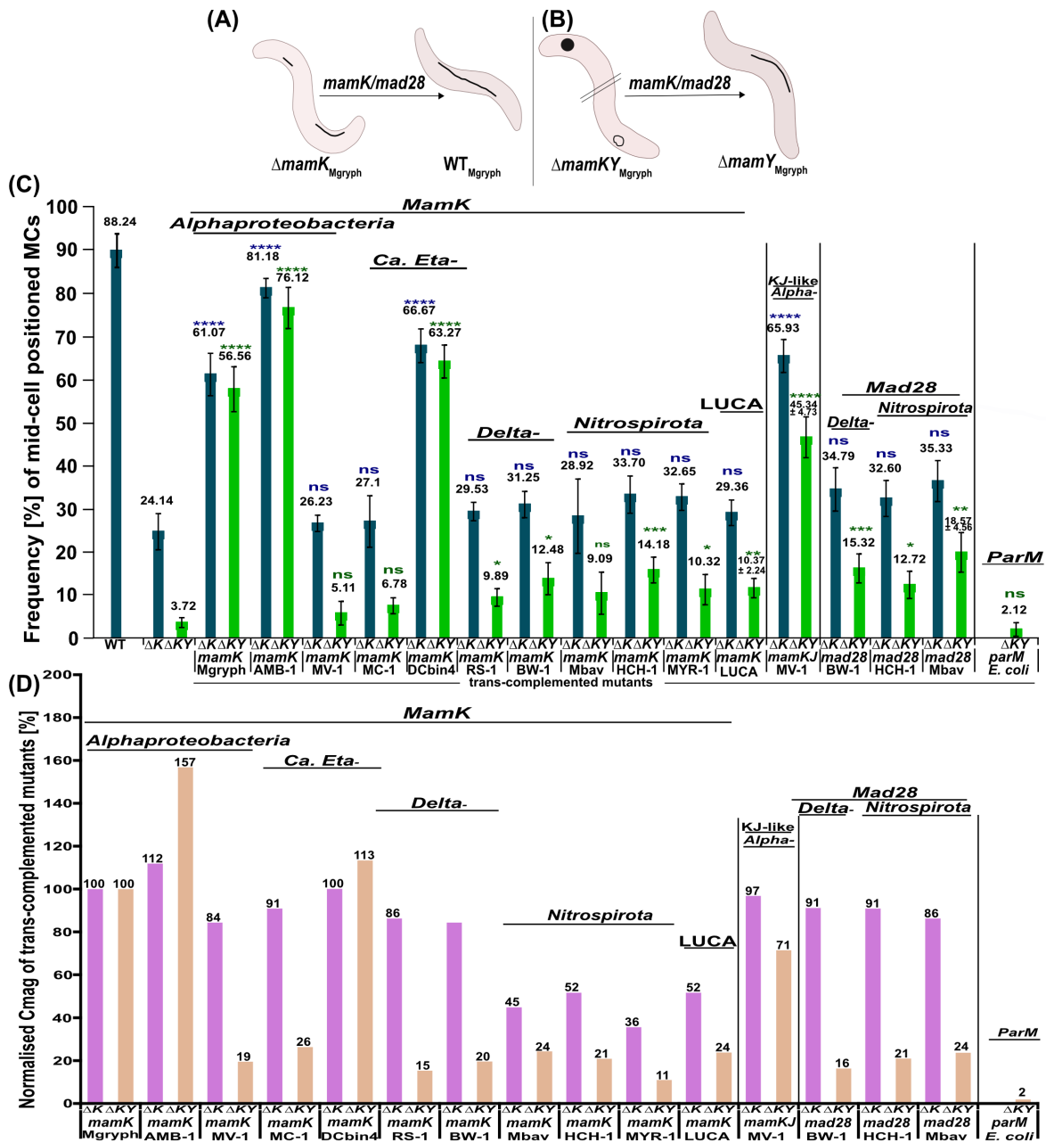
FIG 2 (A and B) Schematic representation of magnetosome organization in WT Mgryph and the magnetoskeleton mutants \Delta mamK_{Mgryph} , \Delta mamKY_{Mgryph} , and \Delta mamY_{Mgryph} . WT Mgryph , magnetosomes organized in straight chains that run along the geodetic cell axis; \Delta mamK_{Mgryph} , short, fragmented, off-center chains; \Delta mamKY_{Mgryph} , agglomerated magnetosomes or magnetic flux-closed rings; \Delta mamY_{Mgryph} , magnetosome chain at the negative inner cell curvature. Arrows indicate expected reconstitution of magnetosome chain organization in case of successful trans-complementation with mamK from diverse MTB in \Delta mamK_{Mgryph} (A) and in \Delta mamKY_{Mgryph} (B). (C) Degree of complementation as inferred from MC organization in \Delta mamK_{Mgryph} and \Delta mamKY_{Mgryph} . Blue bars, frequency of magnetosome chains positioned at mid-cell in WT Mgryph , \Delta mamK_{Mgryph} , and \Delta mamK_{Mgryph} that was complemented with the indicated genes. Green bars, frequency of magnetosome chains (>10 particles, resembling \Delta mamY_{Mgryph} phenotype) in \Delta mamKY_{Mgryph} and \Delta mamKY_{Mgryph} that was trans-complemented with the indicated genes. The numbers of analyzed cells (N) correspond to >200. All values are expressed as mean \pm standard error of the mean (SEM). Statistical significance is indicated as follows: * P \leq 0.05 , ** P \leq 0.01 , *** P \leq 0.001 , **** P \leq 0.0001 , and non-significant (ns) when P > 0.05 . Statistical significance was assessed using a non-paired t-test between the control strains ( \Delta mamK_{Mgryph} in blue and \Delta mamKY_{Mgryph} in green) and the corresponding trans-complemented mutants in the control strains. (D) Relative magnetic response ( C_{mag} ) of complemented \Delta mamK_{Mgryph} and \Delta mamKY_{Mgryph} strains. The C_{mag} of Mgryph strains that were complemented with the native allele was set to 100%, and the C_{mag} of the strains with diverse mamK s, mamK LUCA , mamKJ -like MV-1 , mad28 , and parM genes was normalized to the respective value to obtain the relative C_{mag} as indicator for functional complementation. The values of C_{mag} were derived from four independent Tn5 insertion mutants.
