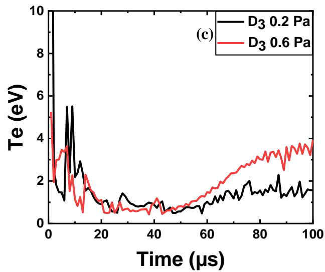
Figure 10. Influence of the pressure on the electron temperature for different pulse sequences (a) D 1 , (b) D 2 and (c) D 3 given in Table 2.
