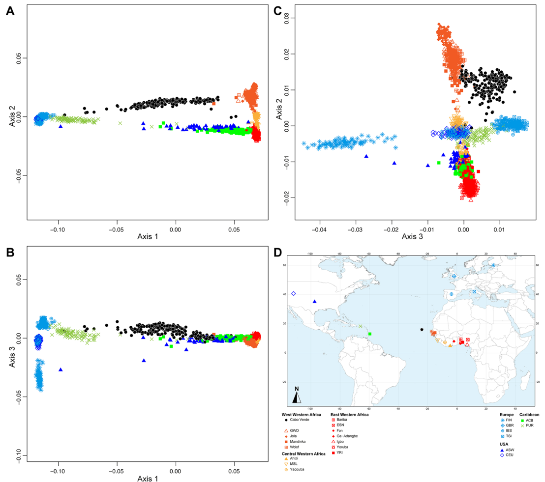
Appendix 2—figure 4. Multidimensional scaling three-dimensional projection of allele sharing pairwise dissimilarities, for the closest subsets of West African, European and other admixed populations related to the TAST. Each individual is represented by a single point. We removed all West and South-West Central African samples, as well as South African samples, compared to the sample set employed in Appendix 2—figure 3 , and recomputed the MDS based on this reduced sample set. See Figure 1—source data 1 for the population list used in these analyses. Sample map used in these analyses is extracted from Figure 1 and provided in panel D . (A) Axis 1 and 2; (B) Axis 2 and 3; (C) Axis 1 and 3. 3D animated plot is provided in .gif format. We evaluate the Spearman correlation between 3D MDS projections and the original ASD pairwise matrix to evaluate the precision of the dimensionality reduction along the first three axes of the MDS. We find Spearman \rho of 0.9636 ( p < 2.2 \times 10^{-16} ).
