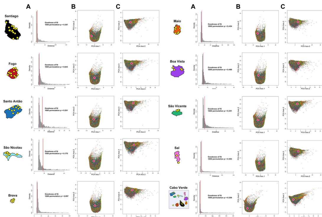
Appendix 1—figure 3. ABC Prior-checking for Methis simulations for each island separately. 10,000 simulations are conducted under each four competing scenarios of historical admixture considered in Random-Forest ABC scenario-choice (see Figure 6 ). (A) Goodness-of-Fit tests: we use as goodness-of-fit statistic the median of the distance between one target vector of 42 summary-statistics and the vectors of 42 statistics obtained for the 1% simulations in the 40,000 simulations reference table that are closest to the target (as identified by simple rejection Pritchard et al., 1999 ). Results obtained with the observed data as target are indicated in the vertical red line. Null-distribution of the goodness-of-fit statistics as histograms are obtained by considering as target in-turn 1000 random simulations as pseudo-observed data, for each island and for the 225 Cabo Verde-born individuals grouped in a single random-mating population, separately. (B) First two axes of a principal component analysis performed on the 42 summary-statistics obtained for 40,000 simulations per island (10,000 simulations for each of four competing-scenarios). Each point corresponds to a single simulation colored per scenario: simulations under Scenario 1 are in blue; Scenario 2 in green; Scenario 3 in red; and Scenario 4 in yellow ( Figures 6–7 ). The pink white-circled dot corresponds to the vector of summary-statistics from the observed dataset. (C) Axes 1 and 3 of the same PCA projection as in panel B.
