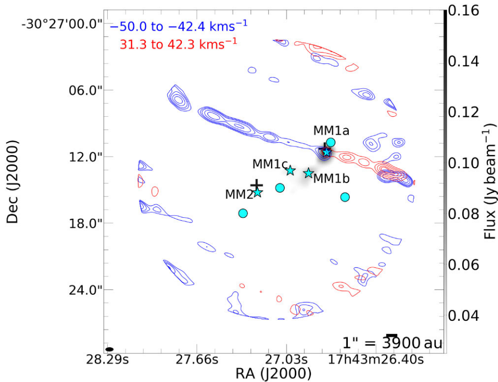
Figure 5. Collimated bipolar outflow of MM1a traced by ^{12}\text{CO} emission. The blue and red contours that indicate the blueshifted ( -50.0 to -42.4 \text{ km s}^{-1} ) and redshifted ( 31.3 to 42.3 \text{ km s}^{-1} ) emission, respectively, are superimposed on a grey scale image of the dust continuum. The position of the 6.7 GHz methanol maser sources are indicated by the black crosses. Cyan filled circles and cyan stars are the same as in Fig. 3. The circular pattern with beam dilution shows the primary beam of ALMA. The synthesized beam is shown in the left bottom corner as a black ellipse.
