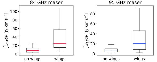
Fig. 9. Integrated intensity for 84 GHz (left) and 95 GHz (right) masers, with and without SiO (2–1) wings. In each box plot the horizontal coloured line represents the median value, the box represents the interquartile range between the 25th and 75th percentiles, and the vertical lines (the ‘whiskers’) show the ranges from the minimum value to the 25th percentile and from the 75th percentile to the maximum value.
