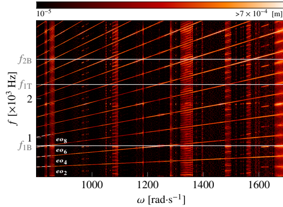
(a) rotor 35
