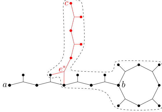
Figure 10: Illustration of Lemma 2.34. The represented objects are T and \mathbf{P}_{V(T)}(c, P_c) . The c -tadpole is highlighted.
