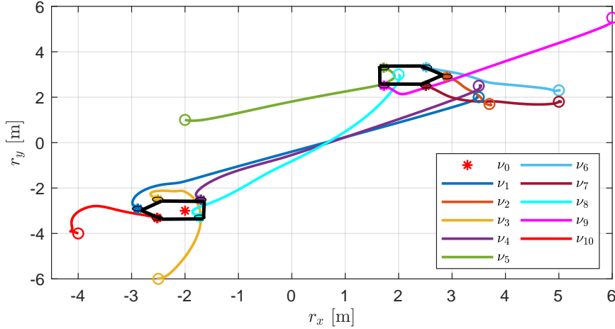
Figure 10. Bipartite formation of system (39) with control input (25). The asterisks are the inertial positions of the robots. The reference points p_i of the mobile robots, on the black circles around the asterisks, of the two disjoint subgroups form a formation around two symmetrical consensus points.
