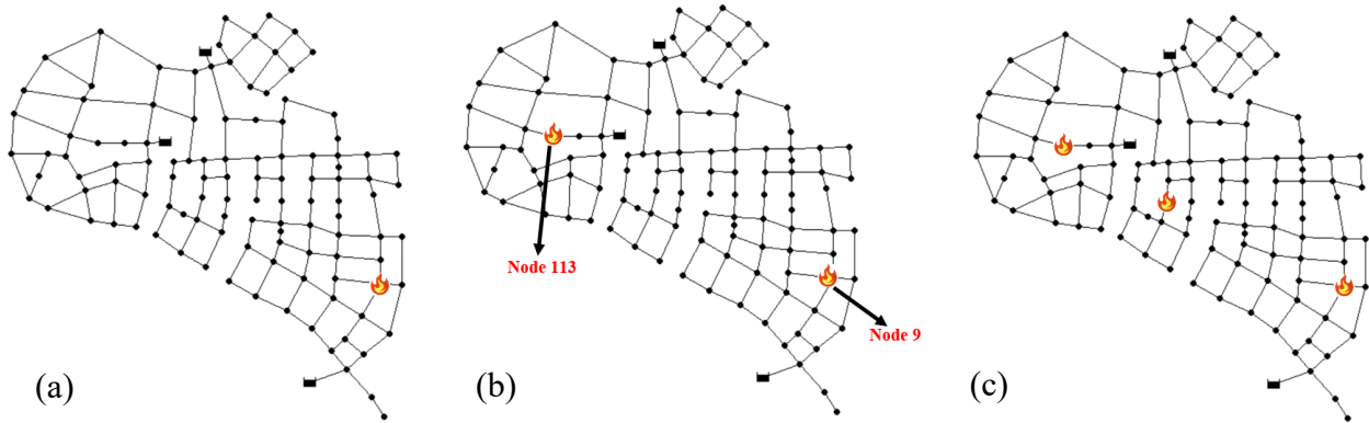
Figure 4. Fire locations for seismic magnitudes of: (a) 5.5; (b) 5.8; (c) 6.0.
