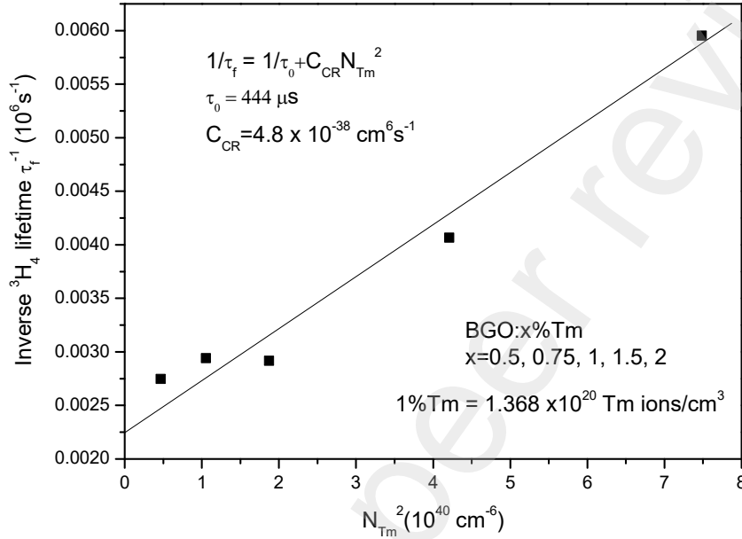
Fig. 8. Plot of the inverse of the average {}^3H_4 \rightarrow {}^3F_4 fluorescence lifetime measured in the singly doped Tm:BGO crystals versus the square of the Tm concentration (with 1\text{at}\%Tm \equiv 1.368 \times 10^{20} \text{ Tm}^{3+} \text{ ions/cm}^3 ).
