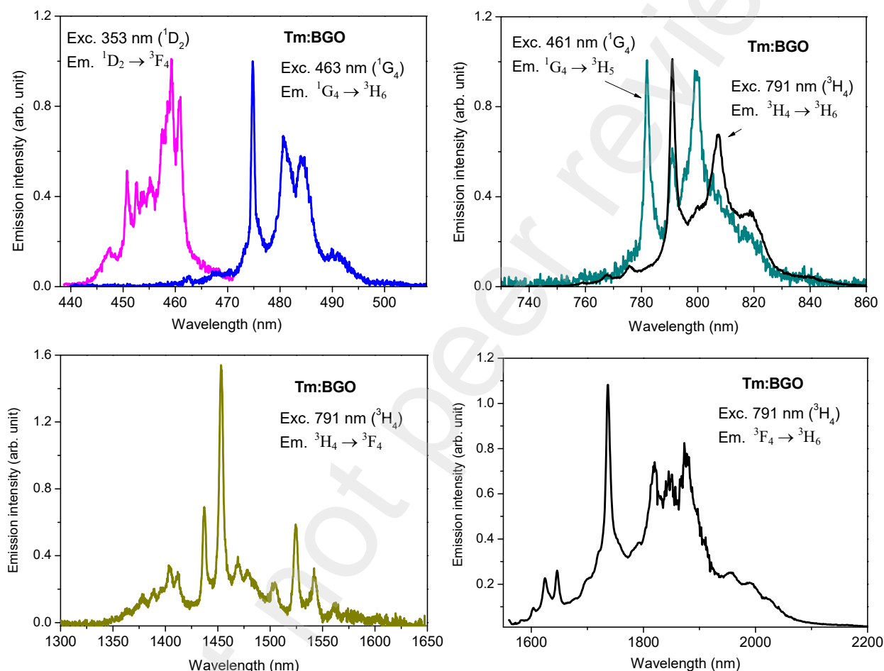
Fig. 6. Emission spectra of 0.5%Tm:BGO registered by exciting the sample at about 353 nm ( ^1D_2 ), 461 nm ( ^1G_4 ) and 791 nm ( ^3H_4 )
