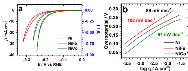
Figure 3. a) Ohmic drop-corrected cyclic voltammograms of Ni, NiFe and NiCo at 5\text{ mV s}^{-1} in KOH 1M. b) Corresponding Tafel plots.
