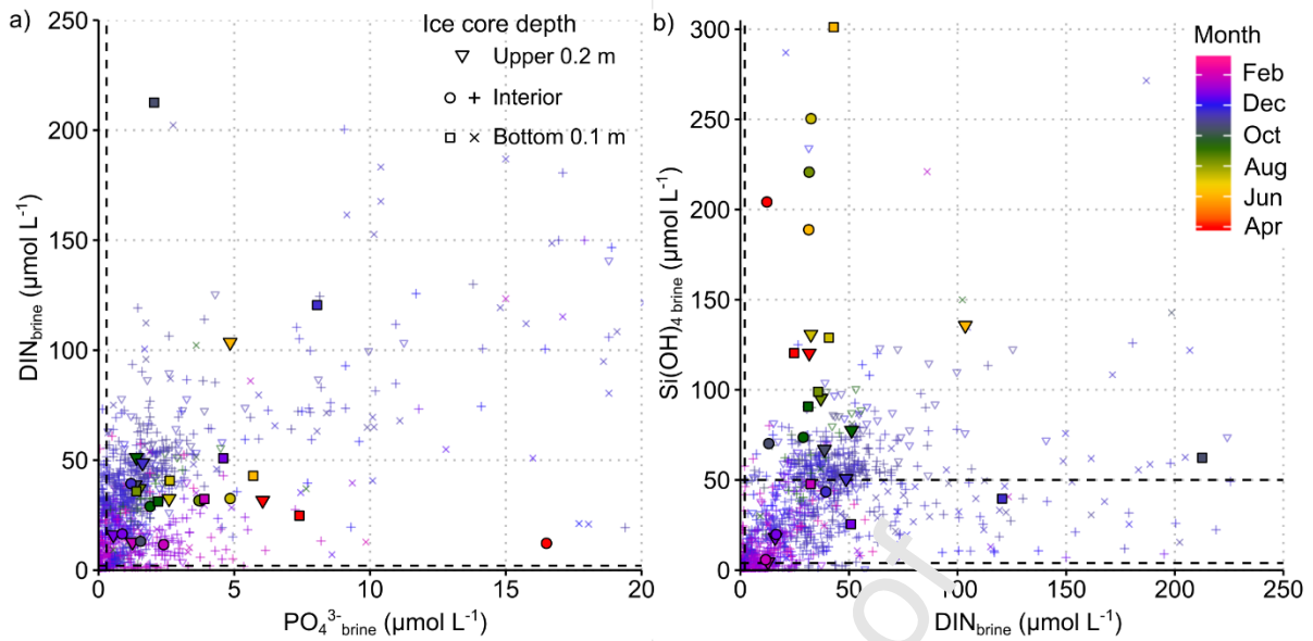
Figure 12. Nutrient-nutrient plots showing estimated individual (smaller open symbols) and monthly median (larger filled symbols) concentrations in fact ice brine from all ice types: (a) DIN-phosphate; (b) silicic acid-DIN. Symbols are colour-coded by sampling date from 1 April (red) to mid-February (magenta) each year, according to the legend. Ice core depth is represented by symbol type as follows: triangles=upper 0.2 m, circles and crosses=interior, squares and x symbols=bottom 0.1 m. Dashed black lines show representative concentrations below which nutrient limitation is known to occur (DIN = 2 \mu\text{mol L}^{-1} ; phosphate = 0.3 \mu\text{mol L}^{-1} ), and measured and estimated values for the nutrient half-saturation constant for silicic acid ( K_{\text{Si}} = 3.9 \mu\text{mol L}^{-1} and 50 \mu\text{mol L}^{-1} , see text for more details).
