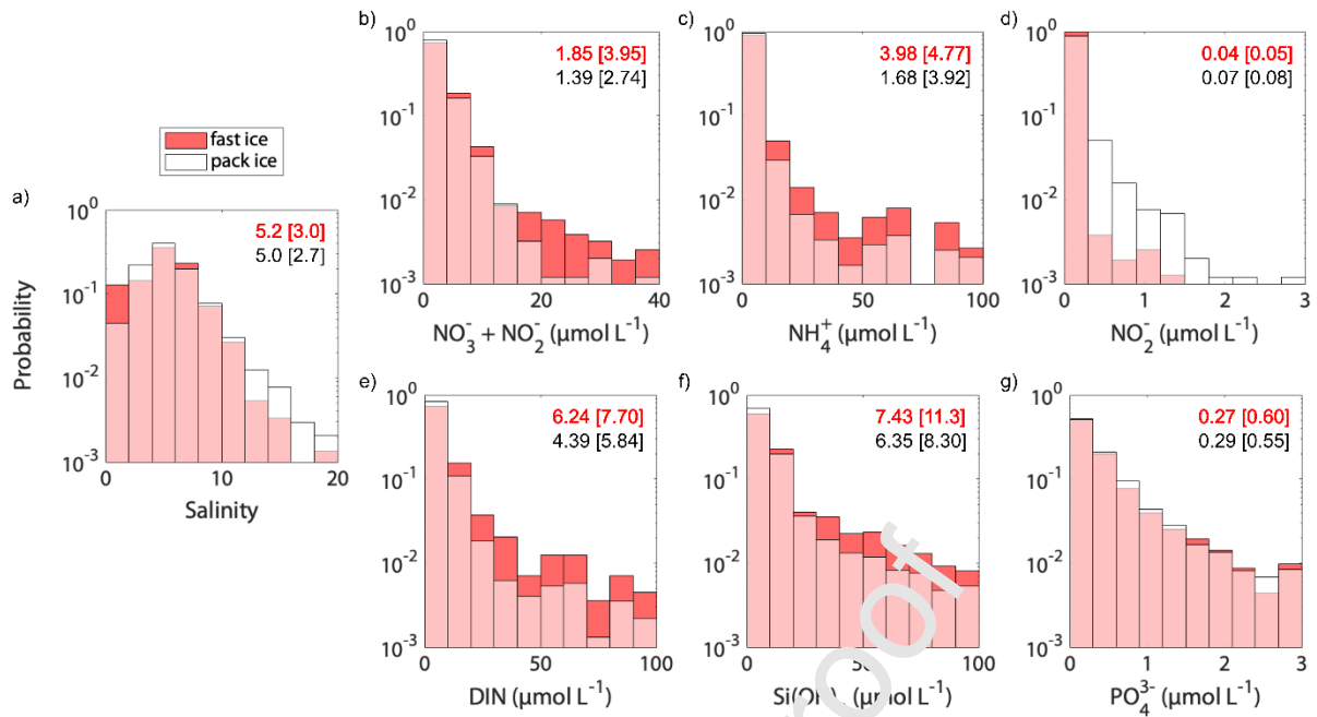
Figure 7. Frequency histograms of measured (a) salinity and concentrations of (b) nitrate, (c) ammonium, (d) nitrite, (e) DIN, (f) silicic acid and (g) phosphate in fast ice (red, this study) and pack ice (white, Fripiat et al., 2017). Values given are medians and interquartile ranges (in square brackets) for each ice environment (red text=fast ice; black text=pack ice).
