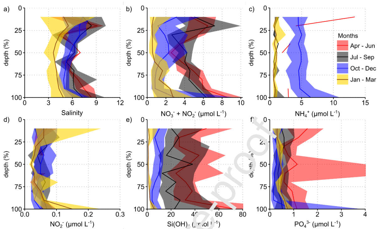
Figure 4. Vertical profiles for bulk salinity and nutrient concentrations in first-year fast ice cores as a function of normalised ice core depth. Data are presented as seasonal averages per three months, where red=AMJ, black=JAS, blue=OND, and gold=JFM (as per legend). Median values and interquartile ranges are shown for (a) salinity, (b) nitrate, (c) ammonium, (d) nitrite, (e) silicic acid and (f) phosphate in bins of 10% of normalised core depth.
