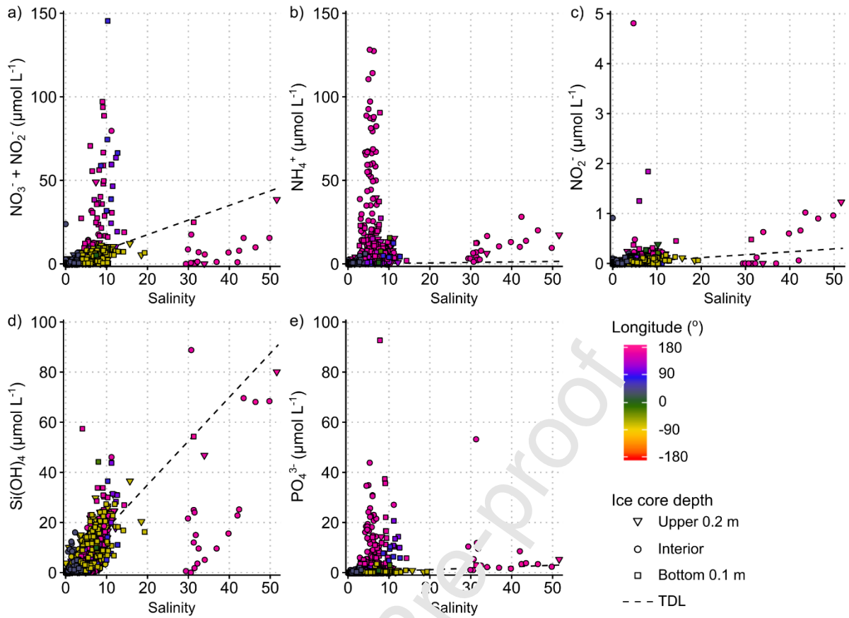
Figure 10. Nutrient-salinity plots for all ice types showing (a) nitrate, (b) ammonium, (c) nitrite, (d) silicic acid, (e) phosphate. Data points are colour-coded by longitude as per legend and the symbols depict ice core depth ( \nabla =upper 0.2 m, \circ =interior, \square =bottom 0.1 m). Dashed black lines are theoretical dilution lines (TDLs) depicting conservative relationships of each nutrient with salinity.
