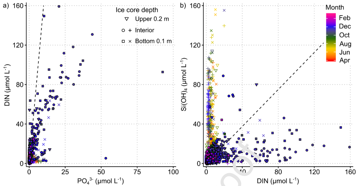
Figure 11. Nutrient-nutrient plots showing measurement from all ice types: (a) DIN-phosphate; (b) silicic acid-DIN. Filled symbols depict when ammonium data were available and show DIN concentrations; open symbols depict when ammonium data were not available to calculate DIN, so nitrate concentrations are plotted instead. Symbols depict ice core depth: triangles=upper 0.2 m, circles and crosses=interior, squares and x symbols=bottom 0.1 m. Data points are colour-coded by sampling date from 1 April (red) to mid-February (magenta) each year, according to the legend. Both legends apply to both plots. Dashed black lines show the expected relationships based on the Redfield N:P ratio and the 1:1 Si:N ratio expected for nutrient uptake by iron-replete diatoms.
