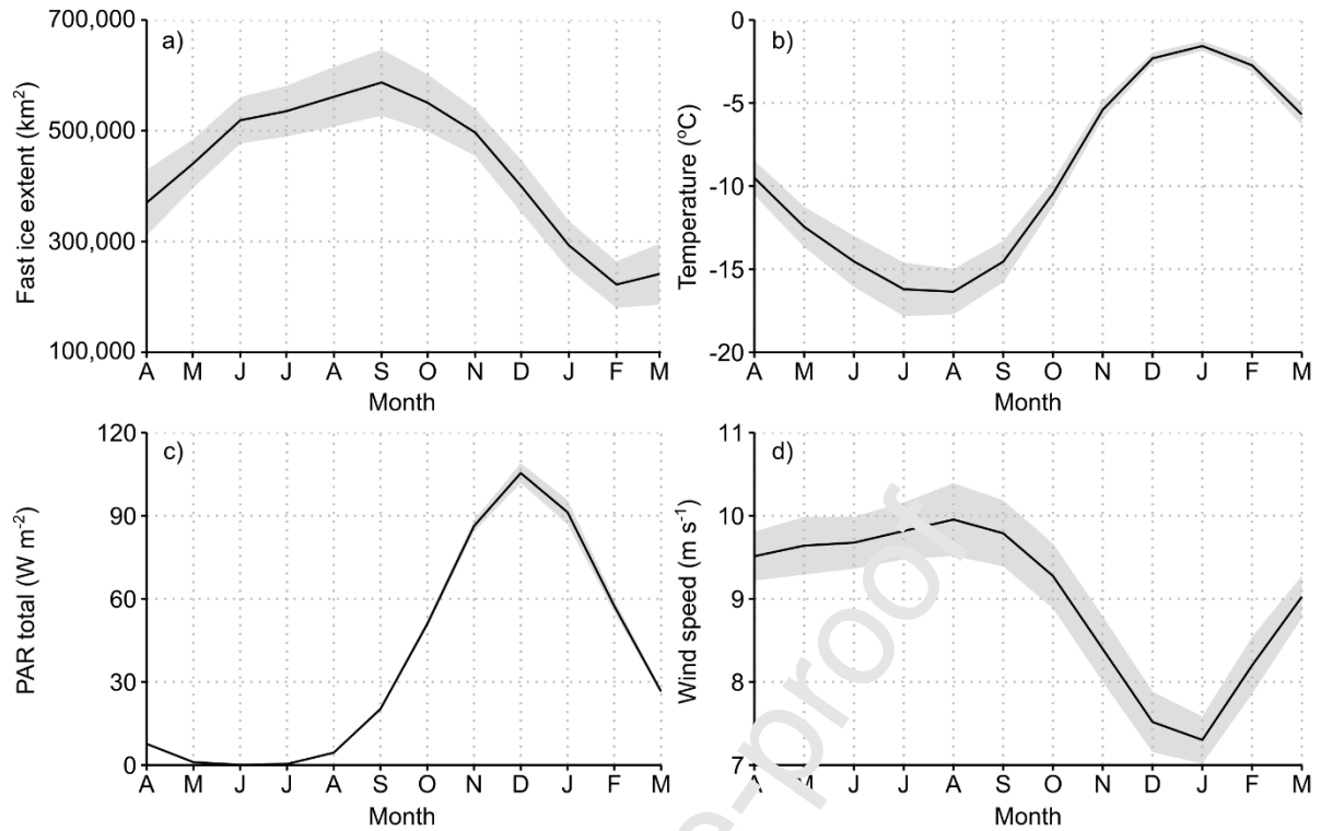
Figure 2. Seasonal patterns of Antarctic fast-ice extent and atmospheric conditions that influence fast ice. (a) Climatology of total fast ice extent showing monthly mean (black lines) and standard deviation (grey shading) values, March 2000 to March 2018 (Fraser et al., 2020; 2021). Also shown are monthly mean (black lines) and standard deviation (grey shading) values for (b) air temperature at 10 m height, (c) total surface downwelling PAR, and (d) surface wind speed, all averaged over the circumpolar ocean region between the Antarctic coastline and latitude 64°S, for 1980-2020, from the MERRA v2 models (Gelaro et al., 2017).
