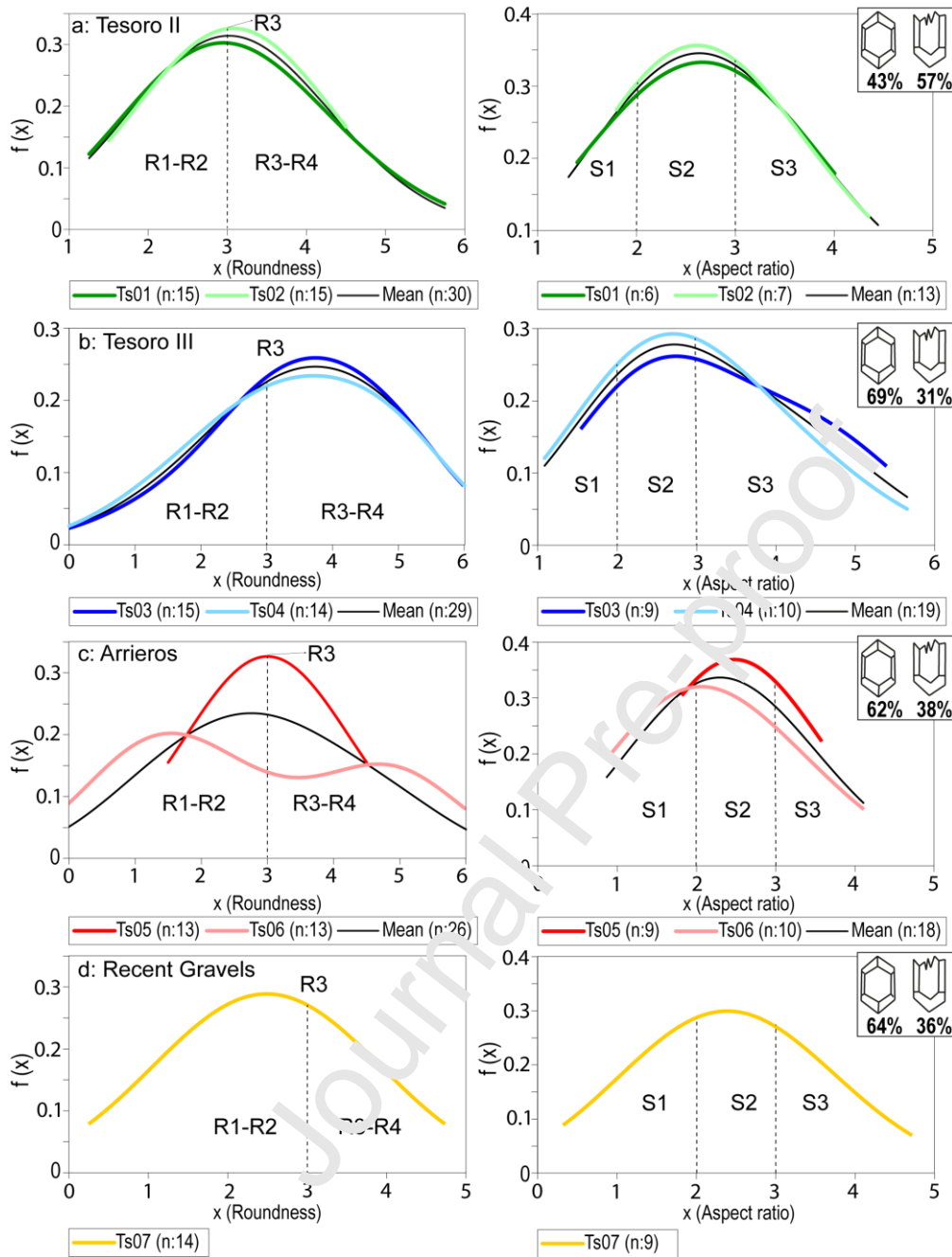
Fig. 4. Kernel density plots of roundness and aspect ratio (length/width) of detrital zircons from the sedimentary record of Centinela District. a Tesoro II gravels. b Tesoro III gravels. c Arrieros gravels. d Recent gravels. Percentage of fractured and non-fractured zircons (right upper corner). S1: aspect ratio <2, S2: aspect ratio between 2 and 3, and S3: aspect ratio >3. n, number of analysed crystals.
