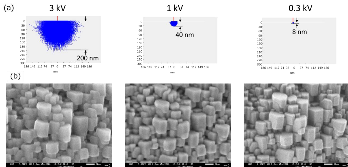
Figure 2. (a) Simulation result of interaction volume of incident electrons in the silicon using Monte Carlo simulation method (Calculated as SiO 2 ). (b) Comparison of SEM images of ZSM-5 obtained at different accelerating voltage: 3 kV, 1 kV, and 0.3 kV.
