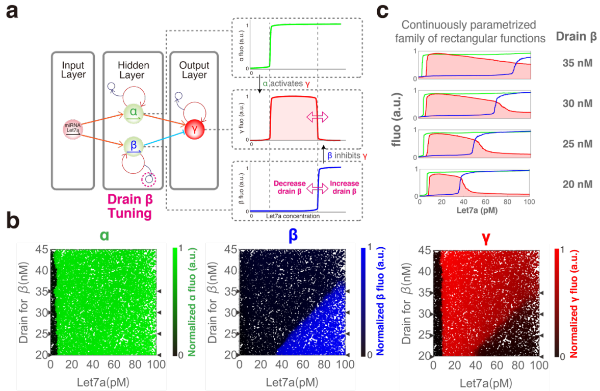
Fig. 4 Synthesis of a parametric family of rectangular functions with a multilayer perceptron. a , A microRNA input activates two neurons ( \alpha and \beta ) in the hidden layer. The output neuron \gamma is activated by \alpha and inhibited by \beta . As a result of these opposing actions, \gamma is only active when \alpha is active and \beta inactive – producing a rectangular function on the input. b , Droplet microfluidic scanning of the concentration of input and a parameter of the network (the concentration of drain for \beta ). The steady state fluorescence of \alpha , \beta and \gamma (after 14h) are shown against the concentrations of let7a and \beta drain. c , Smoothed horizontal slices in the \gamma plot (gray arrows) reveal the tunable rectangular function.
