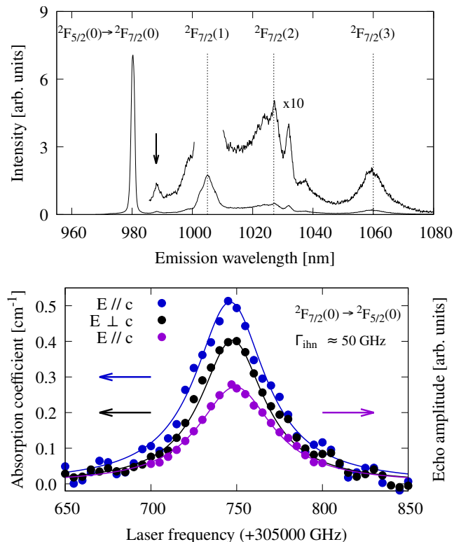
FIG. 2. (Top) Emission spectrum recorded at 11 K exciting the 50 ppm ^{171}\text{Yb}:\text{LN} bulk crystal at 957 nm. Transitions are labelled according to Ref. 51. The peak indicated by the arrow is believed to originate from the coupling with a localized phonon mode. (Bottom, blue and black circles, left scale) Polarized absorption spectra at 10 K. Center frequency corresponds to 980.5 nm (vac.). (Bottom, purple circles, right scale) Photon echo amplitude as a function of the laser frequency at 1 K. The delay between the excitation and rephasing pulses was fixed at 5 \mu\text{s} . Lines represent Lorentzian fits.
