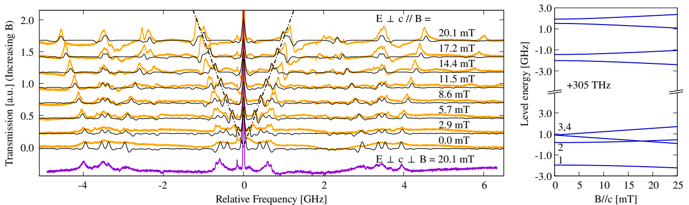
FIG. 4. (Left) Experimental (orange) and simulated (black) optical SHB spectra for different external magnetic fields oriented along the c axis. In purple, the spectrum acquired with the maximum magnetic field (20.1 mT) directed perpendicular to the c axis. A vertical shift has been added for clarity. The dotted lines highlight the linearly shifting holes attributed to ^{171}\text{Yb}^{3+} ions in \text{C}_3 sites or impurities of even \text{Yb}^{3+} isotopes. The narrow peak at -160 MHz is an artifact caused by an AOM. Experiments were performed at 1 K. (Right) Simulated ^2\text{F}_{7/2}(0) and ^2\text{F}_{5/2}(0) hyperfine level energies as a function of magnetic field along the c axis.
