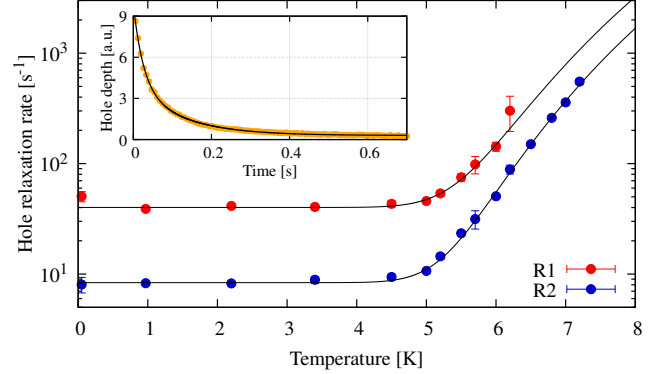
FIG. 6. (Inset) Optical hole depth as a function of delay after burning ( T = 1 K). (Main) Temperature dependence of the two hole relaxation rates (circles) and fit using Eq. 4 (lines).
