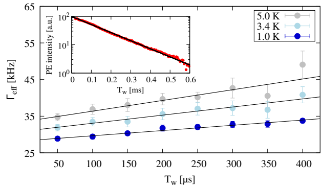
FIG. 8. Three-pulse photon echo experiments. (Main) Effective homogeneous linewidth estimated from Eq. 7 vs. waiting time at three temperatures. The black lines are linear fits. (Inset) Photon echo peak intensity as a function of waiting time for \tau_d = 2.5 \mu\text{s} and at T = 1 \text{ K} . The black line is a fit using Eq. 7.
