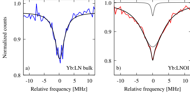
FIG. 5. (a,b) Optical spectral holes burnt in ^{171}\text{Yb} :LN bulk crystal and ^{171}\text{Yb} :LNOI waveguide. Linewidths (FWHM) determined by Lorentzian fits (black lines) are 3 MHz (a), and 1 and 9 MHz (b). Experiments were performed at 5 K.
