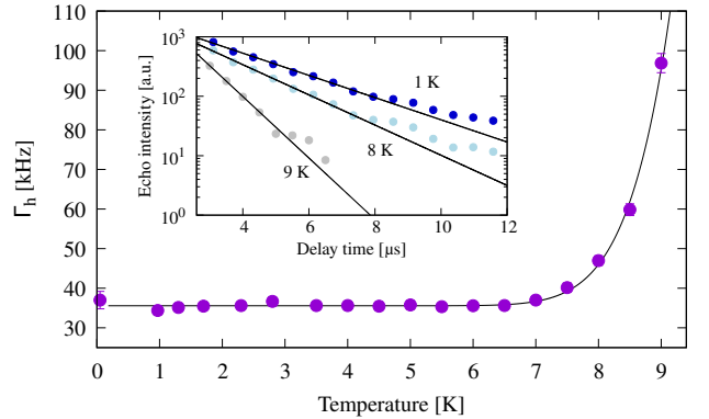
FIG. 7. (Inset) Two-pulse photon echo decay at three differ- ent temperatures. Exponential fits are shown as black lines. (Main) Homogeneous linewidth, obtained through two-pulse photon echo measurements, as a function of temperature (cir- cles) and fit using Eq. 5 (black line).
