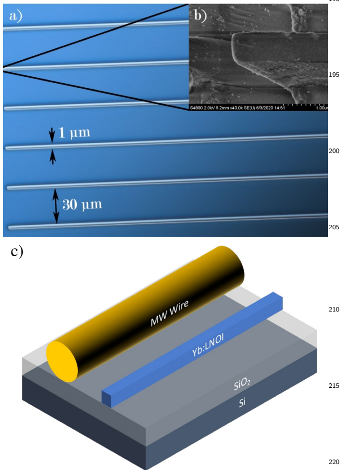
FIG. 1. a) Optical microscope image of LNOI waveguides. b) Scanning electron microscope image of the 45^\circ undercut used to redirect light out of the sample plane. c) A microwave wire was stretched parallel to the waveguide to resonantly drive ^{171}\text{Yb}^{3+} spins.
