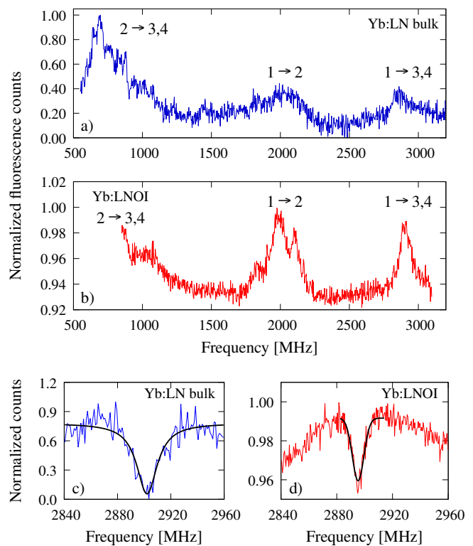
FIG. 3. (a,b) ODMR spectra of ^{171}\text{Yb}:\text{LN} bulk crystal and ^{171}\text{Yb}:\text{LNOI} waveguide. The labels refer to the energy levels in Fig. 4 (right). (c,d) MW spectral holes burnt at 2900 MHz in the 1 \rightarrow 3,4 spin transition in ^{171}\text{Yb}:\text{LN} bulk crystal and ^{171}\text{Yb}:\text{LNOI} waveguide. Linewidths are respectively 19 and 10 MHz FWHM. Black lines represent Lorentzian fits. All experiments were performed at 5 K.
