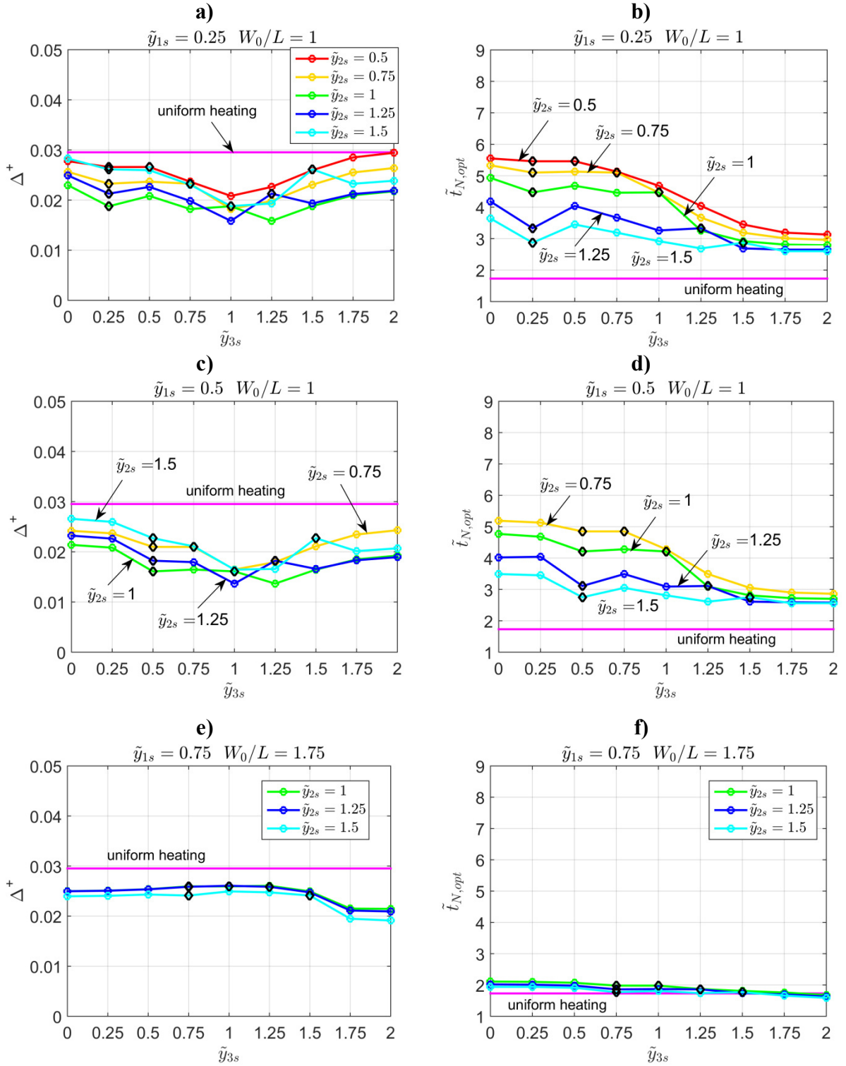
Figure 9. \Delta^+ determinant and \tilde{t}_{N,opt} when using three sensors at \tilde{x} = 0 as a function of the third sensor location \tilde{y}_{3s} with the second one location \tilde{y}_{2s} as a parameter and for the best set-up: \tilde{y}_{1s} = 0.25 and W_0/L = 1 a), b); \tilde{y}_{1s} = 0.5 and W_0/L = 1 c), d); \tilde{y}_{1s} = 0.75 and W_0/L = 1.75 e), f).
