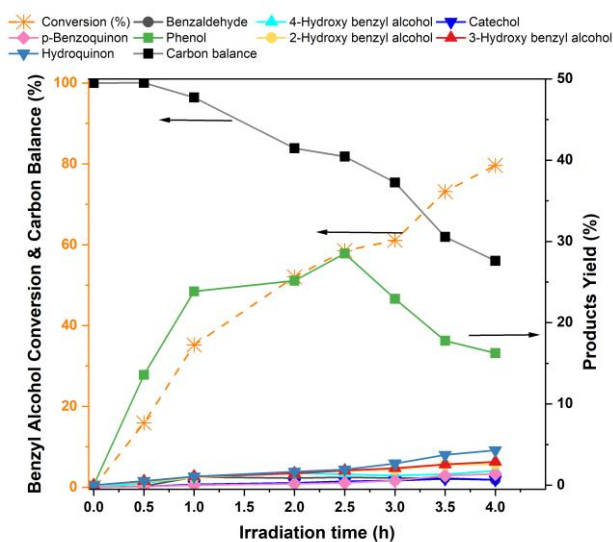
Figure 2. Conversion of benzyl alcohol and products yields in the ultrasound reactor, as a function of time. Reaction conditions: 5 mmol.L -1 Benzyl alcohol, 5.4 mg CuO, 578 kHz, 0.11 W/mL, 25 °C
