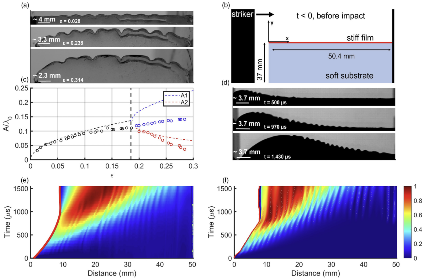
FIG. 1. (a) Pre-impact-test quasistatic compression of sample 1 yields period-doubling behavior. (b) The dynamic test setup. (c) Measured (open circles) and predicted (dashed curves) quasistatic wrinkle amplitude vs strain, corresponding to the test shown in (a). After the critical strain (vertical thick dashed line), the period-doubled mode (blue, top branch) grows, and the original mode (red, bottom branch) fades. (d) Snapshots from a test at 7.1 m/s impactor velocity on a “pristine” sample, displaying multiple-wavelength surface patterns. (e) A normalized spatiotemporal diagram of the experiment shown in (d), with color representing the y -direction surface displacement, U_y . The line visible at the right edge is an artifact of the camera frame edge and should be disregarded. (f) A normalized spatiotemporal diagram of the simulation [7.6 m/s impact velocity, same color scheme as in (e)].
