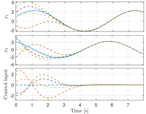
Fig. 3. Distributed consensus of x_1 and x_2 and the control input when the communication graph is a spanning tree.
