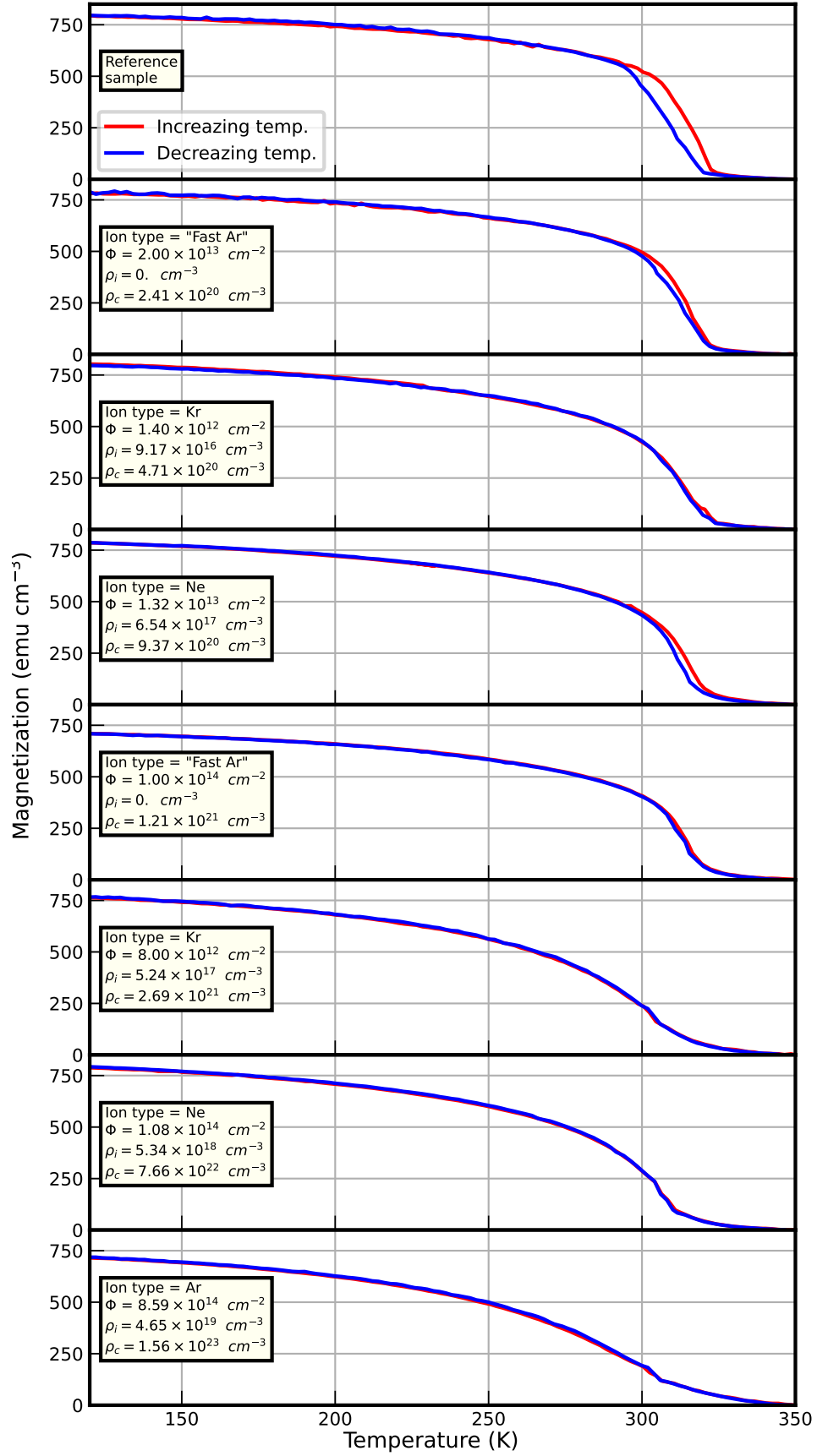
FIG. S1: Isofield ( H = 1 \text{ T} ) magnetization curves M(T) of selected samples. Irradiation details are indicated in the corresponding subplots. Fast ions indicate irradiations with high kinetic energy ions. Irradiation details can be found in Table I.
