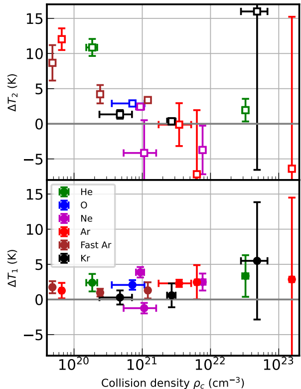
FIG. 5: Differences \Delta T_2 = T_2^h - T_2^c (top), and \Delta T_1 = T_1^h - T_1^c (bottom) between the extrema of the coexistence interval over heating and cooling as function of \rho_c . \Delta T_2 = T_2^h - T_2^c reduces as a function of \rho_c , similarly to \Delta T_{hyst} . \Delta T_1 instead is, on average, close to 0, and does not show any specific trend as a function of \rho_c .
