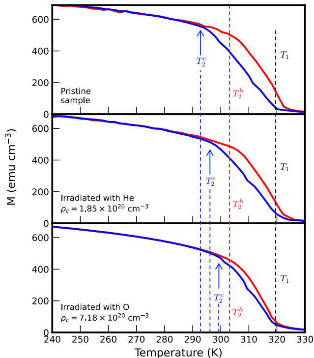
FIG. 4: Comparison between M(T) loops over heating, and cooling (in red and blue), measured on the pristine sample (top), on a He irradiated sample (middle) and on an O irradiated sample (bottom). As apparent from Fig. 5, \Delta T_1 is rather small and does not show any clear trend as a function of the collision density. Thence, a single dashed black line is used to mark T_1 over all the curves. On the contrary, \Delta T_2 reduces as a function of \rho_c . Furthermore, this reduction takes place at fixed T_2^h (i.e. the single dashed red line), with T_2^c getting higher and closer to T_2^h as a function of the collision density (i.e. as shown by the sequence of blue dashed lines in the three frames of the figure).
