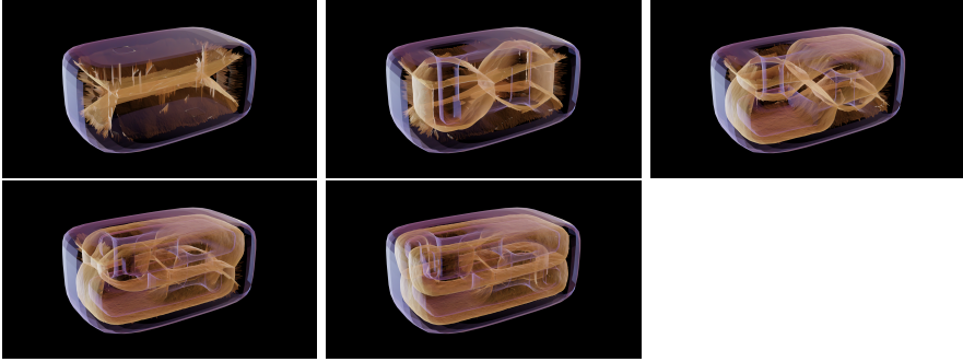
Fig. 9: The evolution of the interior medial axis (yellow) as the smoothed solid cube is deformed into a thickened version of Bing’s house (blue/purple). The smoothed solid cubes in these five frames coincide with the unsmoothed solid cubes in the first five frames of Figure 7. The exact moment at which the medial axis becomes non-collapsible lies between frames four and five and is depicted explicitly in Figure 10.
