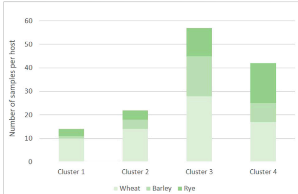
FIGURE 4 Number of Puccinia graminis samples originated from wheat, barley and rye and represented on each of the four clusters identified in the DAPC analysis.
