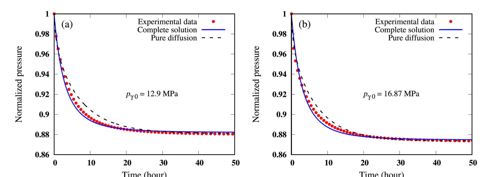
Fig. 4. A comparison between the numerical and the experimental pressure histories for the two laboratory tests: (a) p_{y0} = 12.9 MPa and (b) p_{y0} = 16.87 MPa. The black curves represent the numerical solutions while considering only pure diffusion ( D_{app} = 8.6 \times 10^{-8} m 2 /s)
