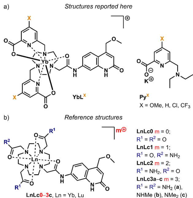
Fig. 2 (a) Complexes studied here ( YbL^X ) and pyridine model compounds ( Py^X ), X is the pyridine p -substituent. (b) Cyclen-based Yb complexes used as the reference structures ( YbLc ), LnLc0–3c are cyclen-based complexes with 0 to +3 overall charge.
