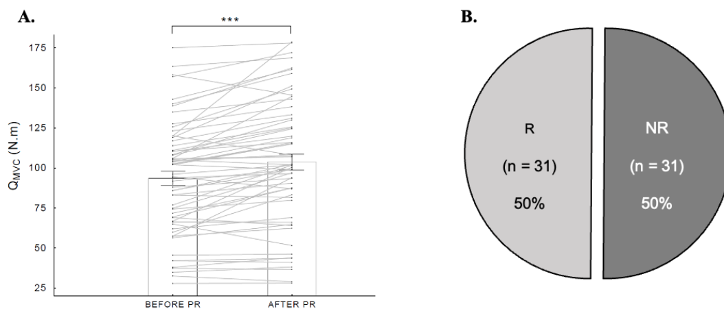
Figure 2. Effects of pulmonary rehabilitation on muscle force:(A) average increase in Q MVC before and after pulmonary rehabilitation; (B) prevalence of non-responders (NR) and responders (R). Abbreviations: R: responders; NR: non-responders; Q MVC : quadriceps maximal voluntary contraction. ***: p < 0.001.
