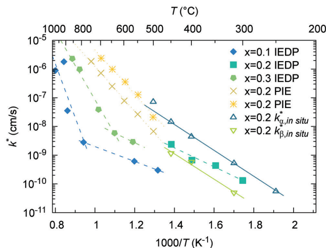
Figure 4. CGO surface exchange kinetics. Tracer surface exchange coefficients as reported in the literature for different types of \text{Ce}_{1-x}\text{Gd}_x\text{O}_2 samples obtained by IEDP or PIE, compared to in situ values found in this work: polycrystalline ceramics ( x = 0.1 and x = 0.2 IEDP [55,56] ), single-crystal CGO ( x = 0.3 IEDP [57] ), and CGO particles ( x = 0.2 PIE [54,58] ).
