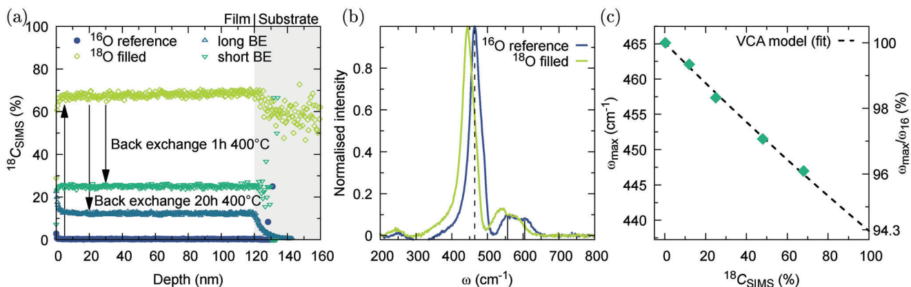
Figure 2. Isotopic Raman shift. a) ToF-SIMS ^{18}\text{O} depth profiles for ^{16}\text{O} annealed reference sample, ^{18}\text{O} exchanged film and two films back-exchanged at 400^\circ\text{C} for 1 and 20 h, respectively. b) ^{18}\text{O} -induced shift as observed by Raman spectroscopy. c) Correlation of Raman shift and the isotopic concentration. The dashed line is the fit of the data to the virtual crystal approximation (VCA).
