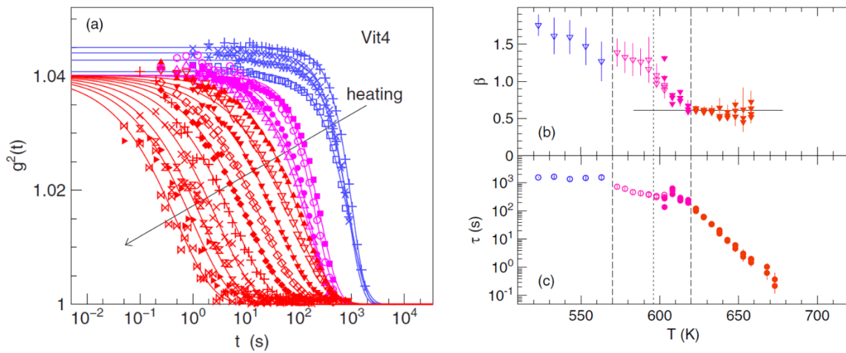
Figure 1. a) Temperature dependence of the correlation functions measured with XPCS in a Vit4 MG during isothermal steps of 5 K between 520K and 675K, obtained by heating the glass with a rate of 1 K/min. The as-cast sample was annealed at 600K prior to the measurements to remove eventual stresses related to the sample preparation. The data are collected at q=2.6\text{\AA}^{-1} corresponding to the first maximum of the atomic structure
