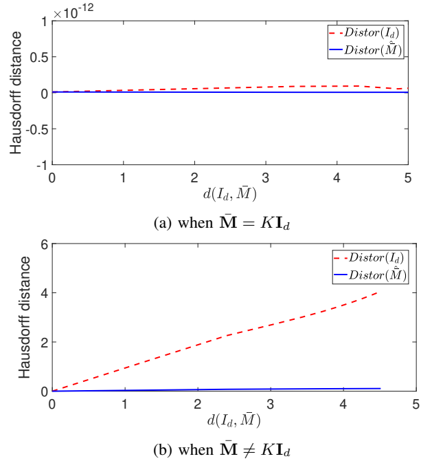
Fig. 1: Hausdorff distance comparison as a function of geodesic distance between \mathbf{I}_d and \bar{\mathbf{M}} .
