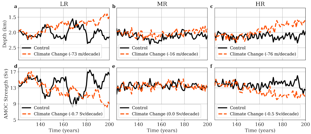
FIG. 4. Time-series of the total AMOC characteristics averaged between 30 and 50^{\circ}\text{N} . The model drift has been removed and the climate change trends indicated in the legends are statistically significant only for the LR and HR. (a-c) Upper cell vertical extent proxy. To follow the depth of the AMOC upper cell in time, we use the depth below 1 km at which the AMOC strength is half of the AMOC strength at year 121, which is the year when the climate change runs branches off from the control runs. We use this metric because it allows us to see changes in the AMOC vertical structure, while there is little change in the depth at which the streamfunction is maximum even if the vertical extent of the cell reduces. We also do not use the depth at which the streamfunction is zero because the lower cell is not well-defined in the LR configuration. The AMOC is interpolated from the coarse model vertical grid to a vertical resolution of 1 meter to determine the depth with accuracy. (d-f) AMOC strength (maximum over the water column in depth coordinates).
