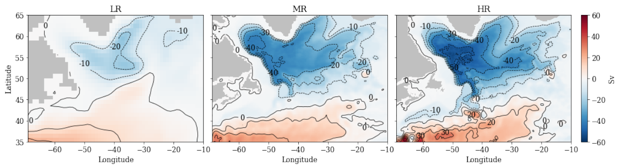
FIG. 11. Barotropic Quasi Streamfunction for the CM2-O model suite, averaged over the last 20 years of the control runs. The grey area is topography
