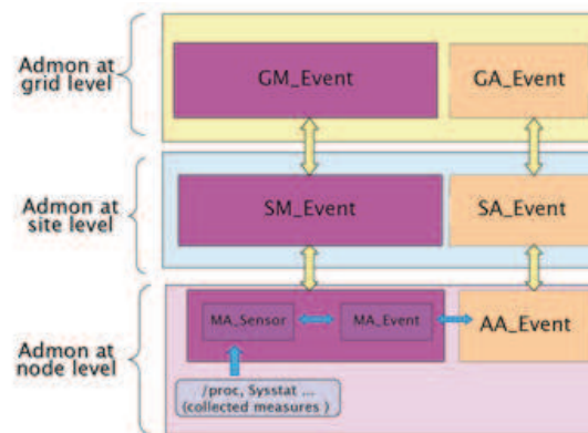
Figure 2: Admon's Architecture
