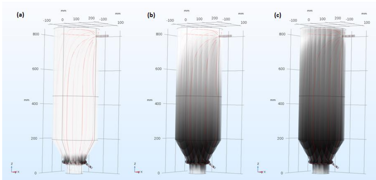
Figure 4. Velocity field inside the reactor (red lines). The black shading represents the moving gas phase distribution as a function of time (a: 1s, b: 50 s, c: 110 s).
