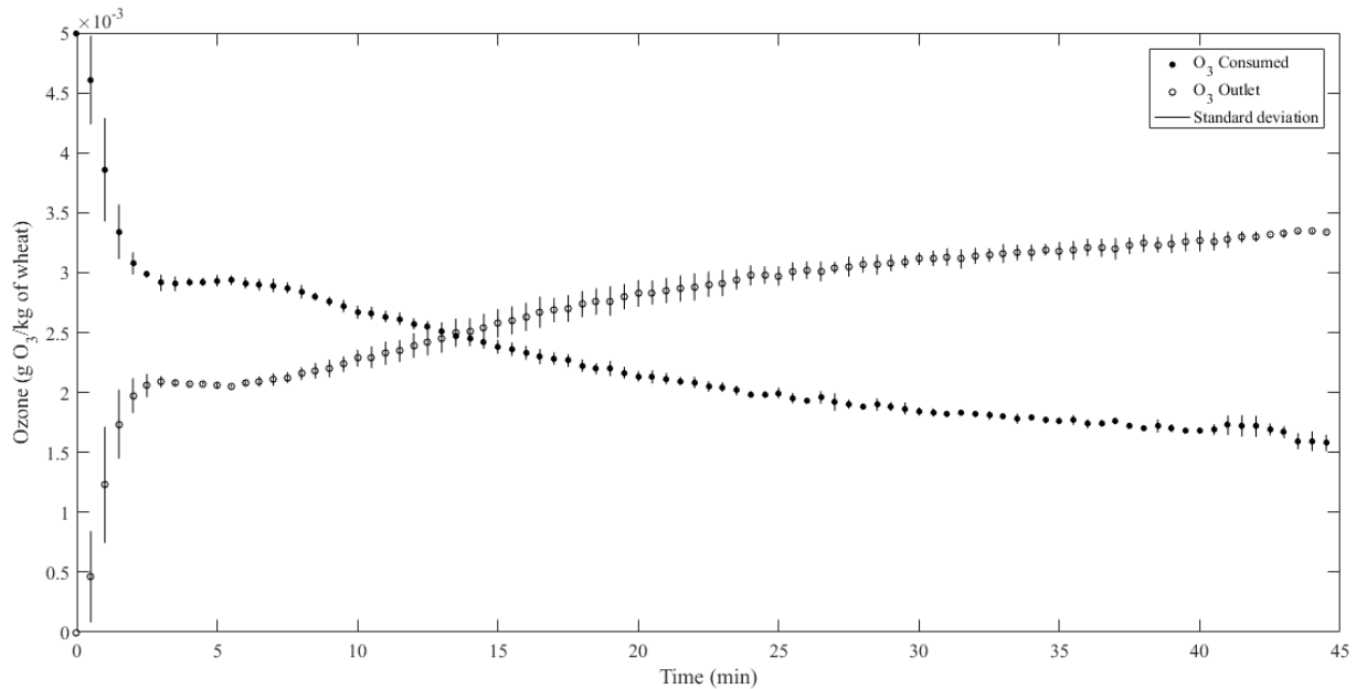
Figure 1. The experimental consumed (●) and outlet (○) ozone with confidence intervals (|)
