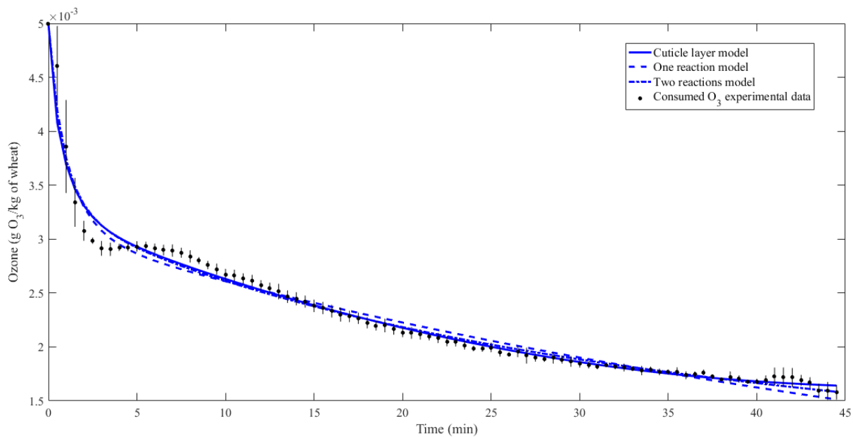
Figure 2. Experimental consumed O 3 with confidence intervals and numerical fitted data using the three models
