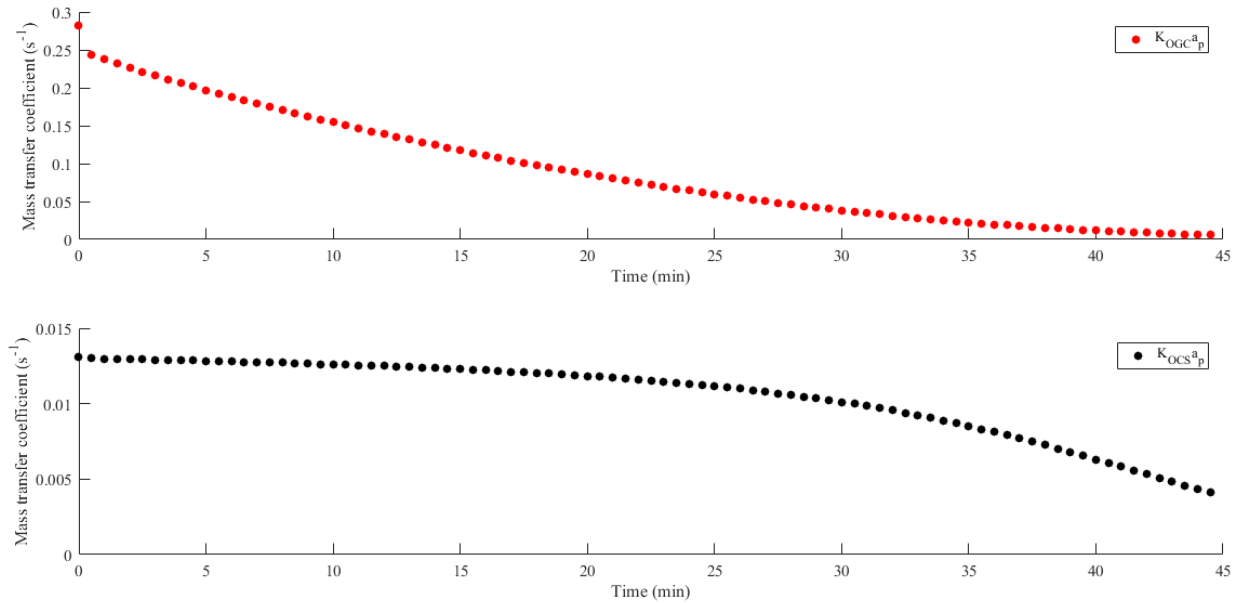
Figure 3. Mass transfer coefficients between gas phase and the cuticle ( K_{OGC}^{a_p} ) and between cuticle and the internal layers of wheat ( K_{OCS}^{a_p} ) as a function of ozonation time
