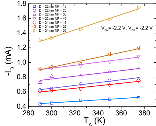
Fig. 2. Drain current as a function of different measurement temperatures, T_{\text{A}} , for the p-type JLNT geometries under study at V_{\text{GS}} = -2.2 \text{ V} and V_{\text{DS}} = -2.2 \text{ V} showing the linear fits associated with each device.
